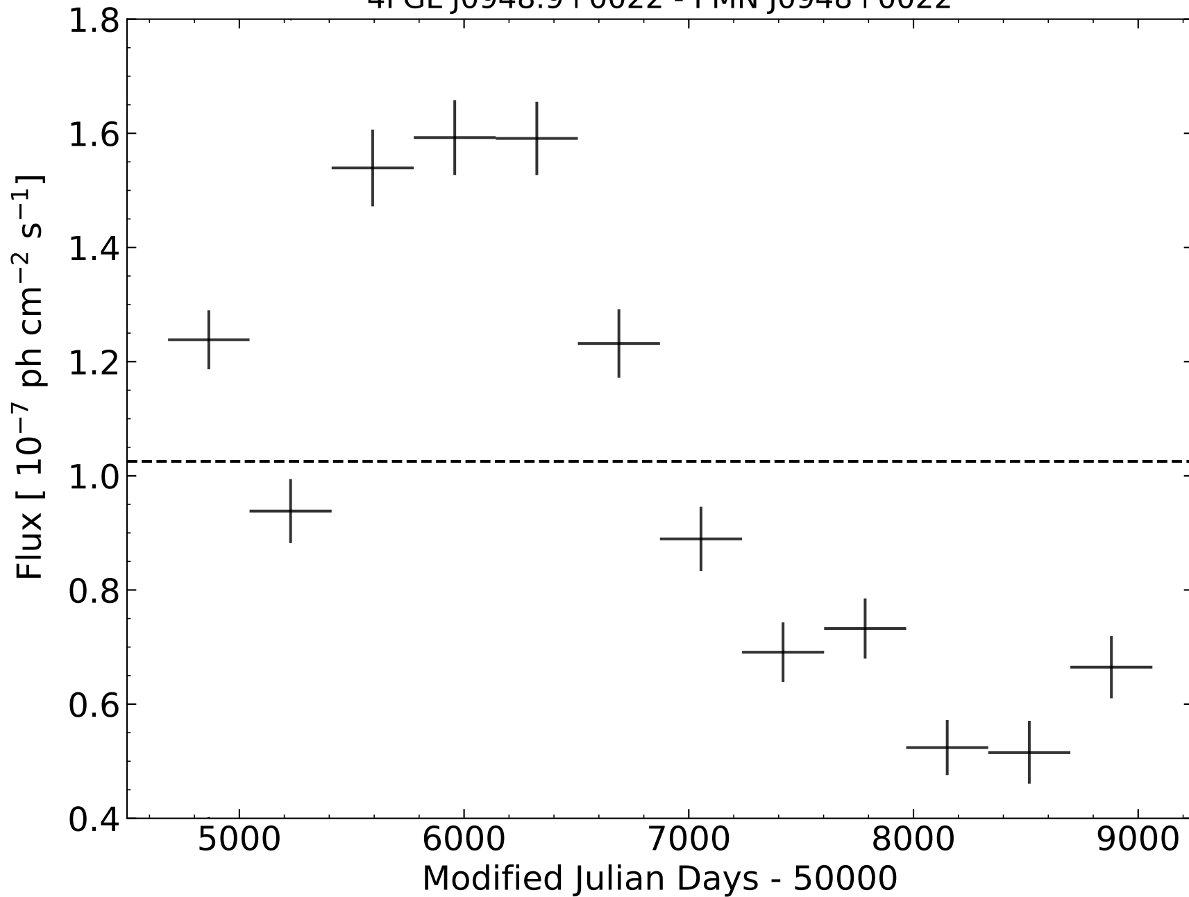
4FGL J0948.9+0022 - PMN J0948+0022
