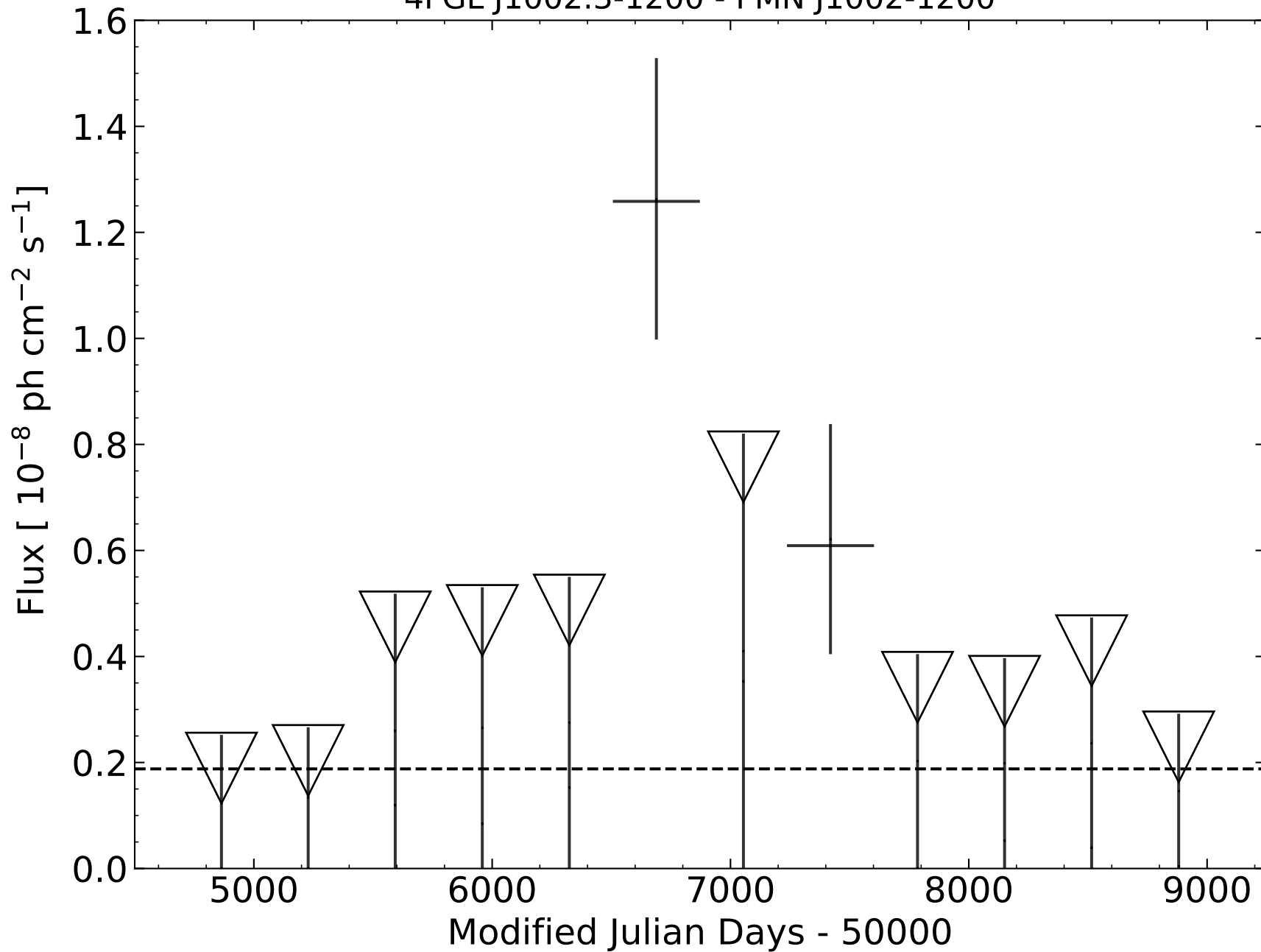
4FGL J1002.3-1200 - PMN J1002-1200
