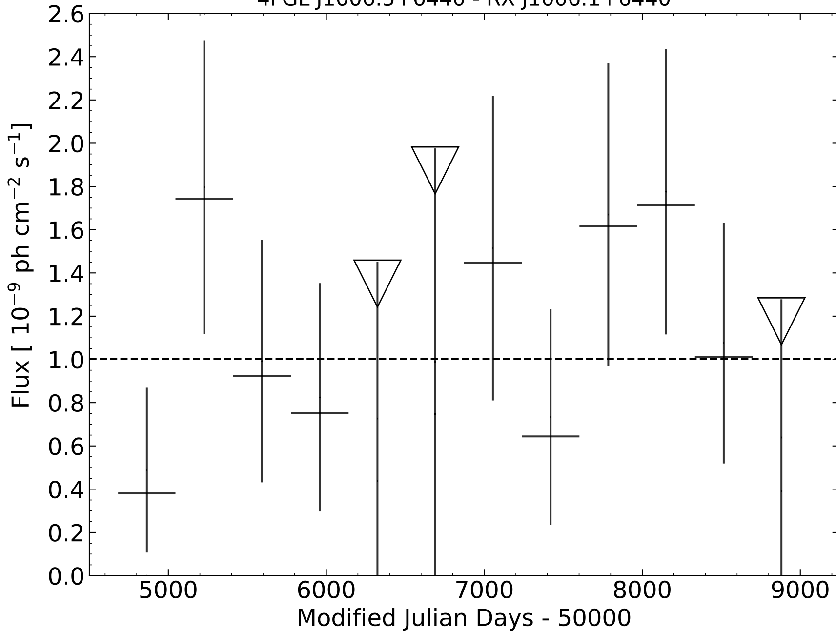
4FGL J1006.5+6440 - RX J1006.1+6440
