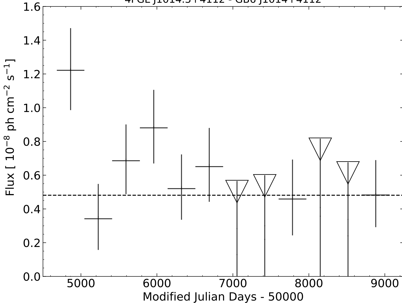
4FGL J1014.3+4112 - GB6 J1014+4112
