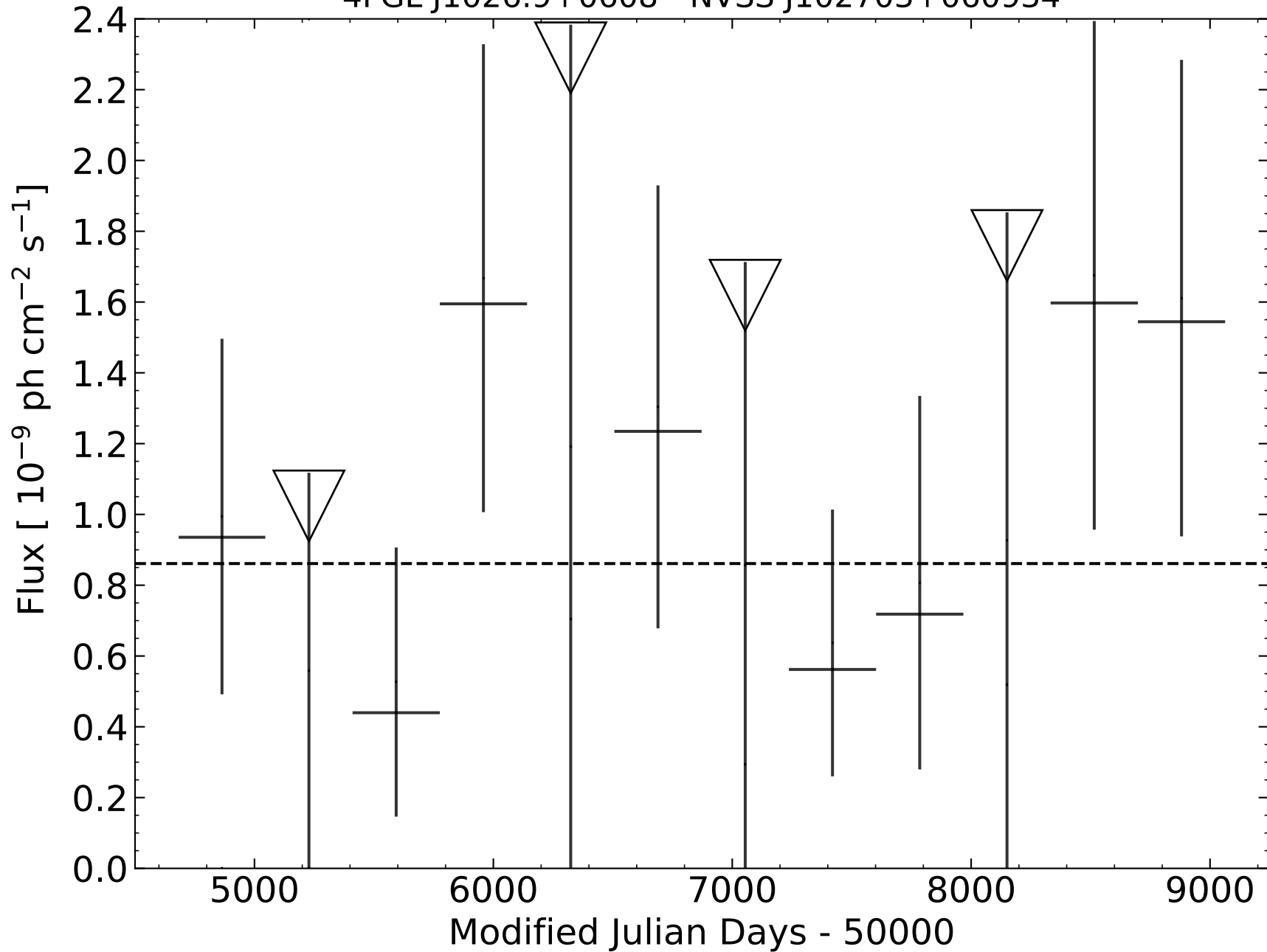
4FGL J1026.9+0608 - NVSS J102703+060934
