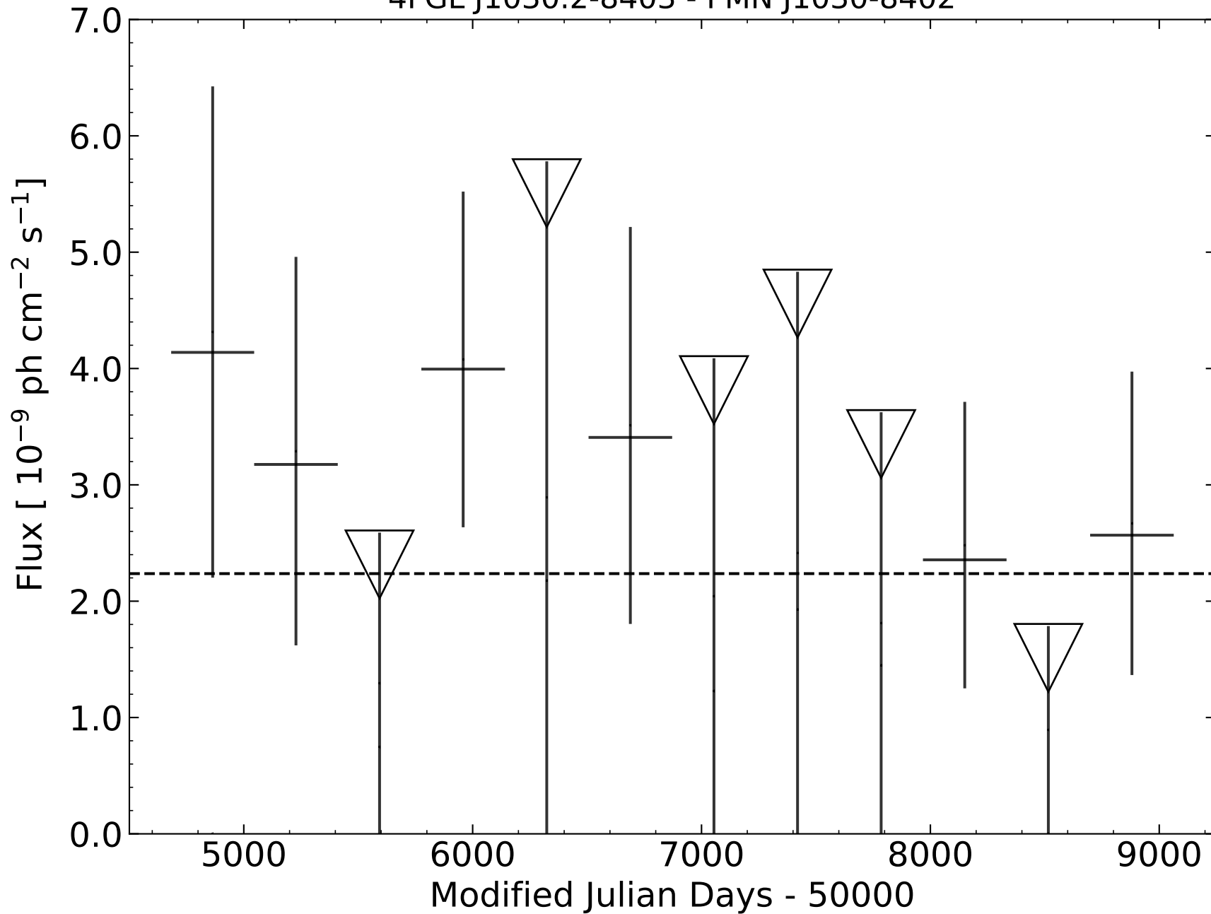
4FGL J1030.2-8403 - PMN J1030-8402
