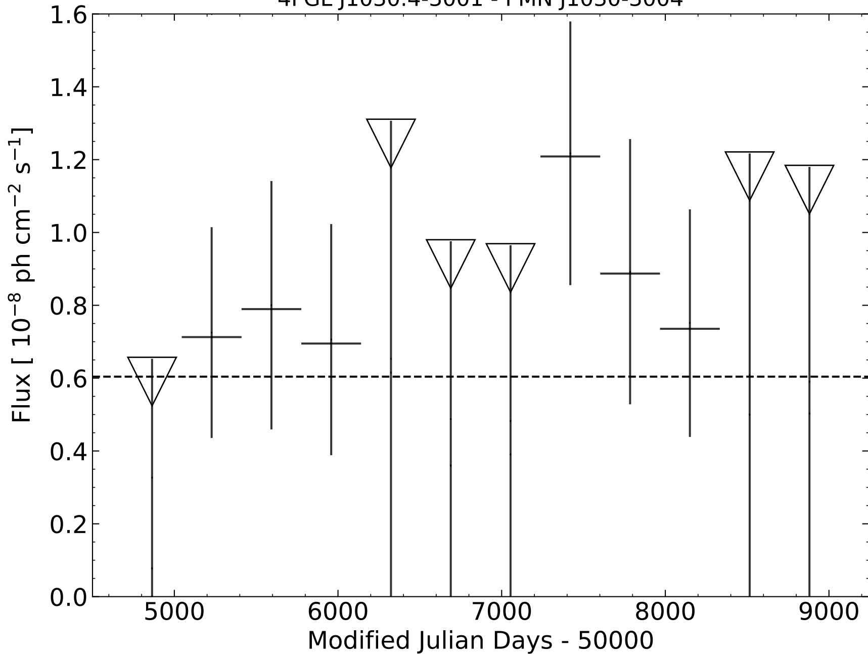
4FGL J1030.4-3001 - PMN J1030-3004
