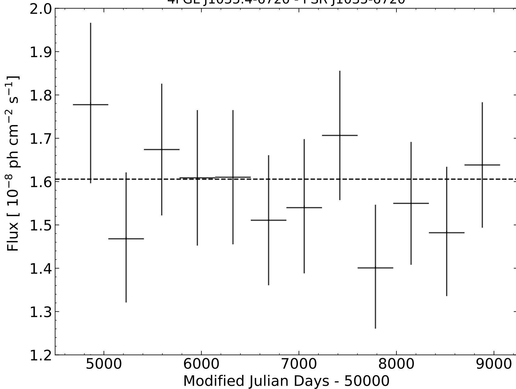
4FGL J1035.4-6720 - PSR J1035-6720
