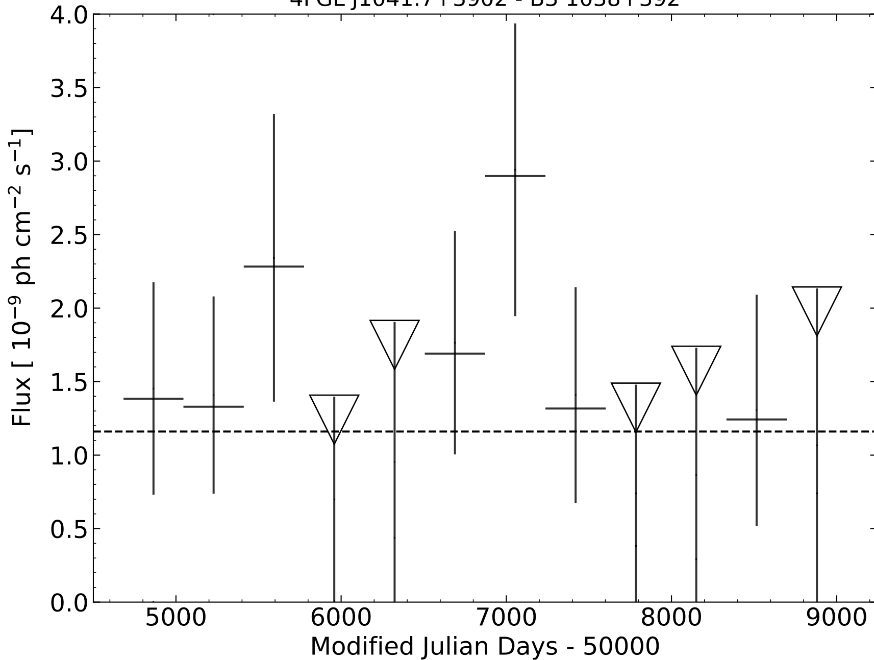
4FGL J1041.7+3902 - B3 1038+392
