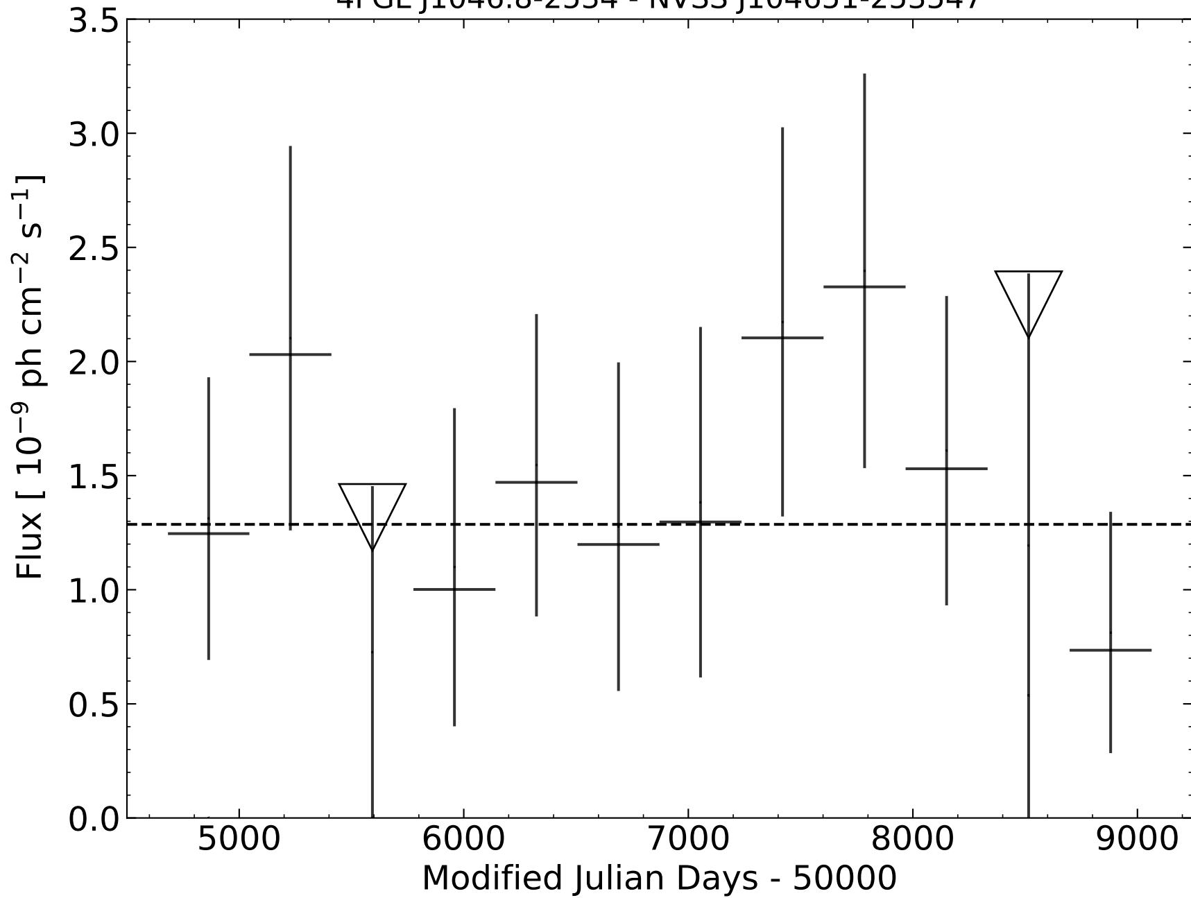
4FGL J1046.8-2534 - NVSS J104651-253547
