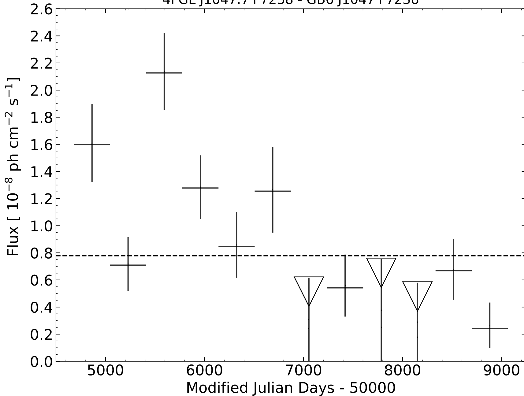
4FGL J1047.7+7238 - GB6 J1047+7238
