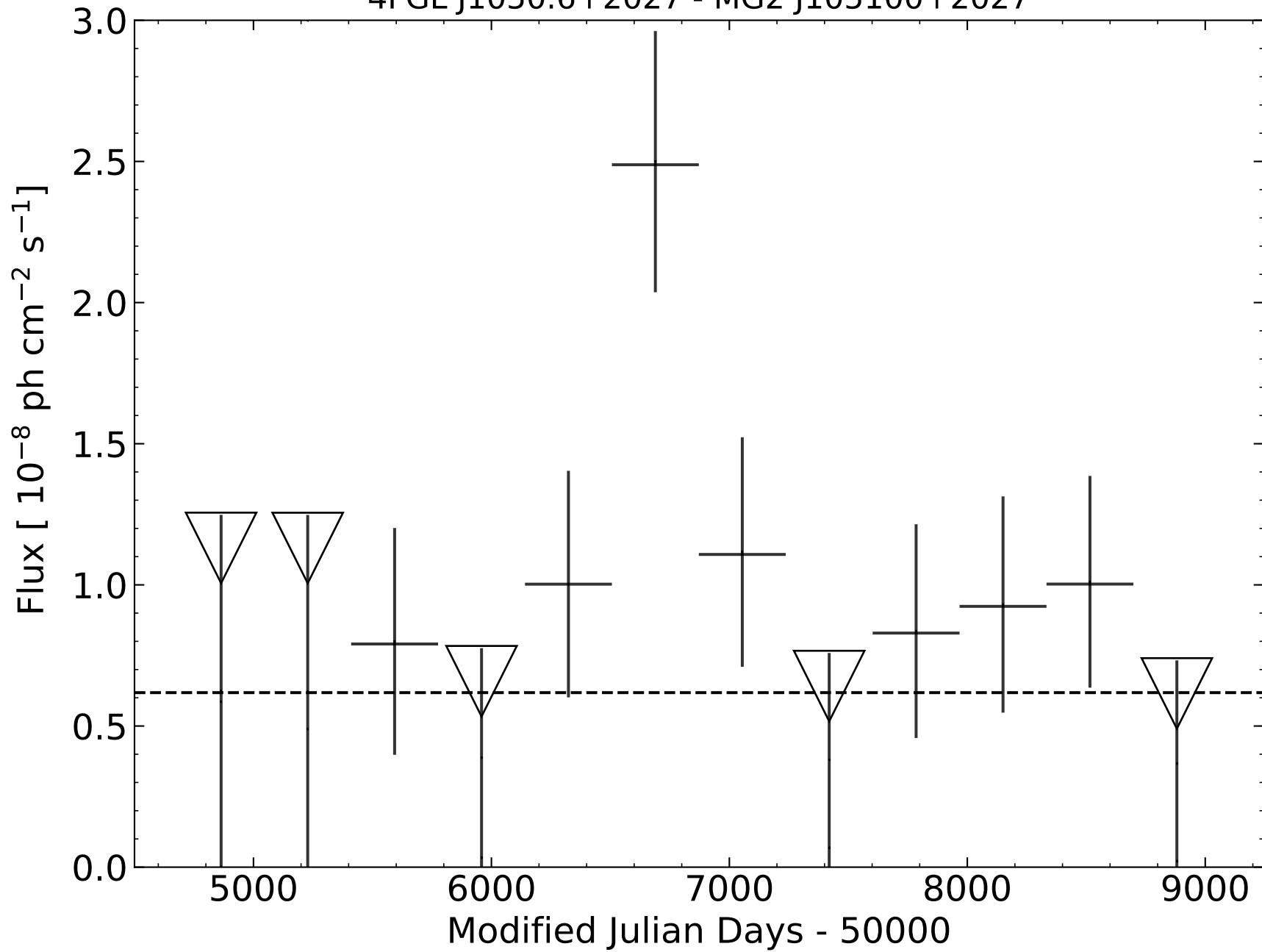
4FGL J1050.6+2027 - MG2 J105100+2027
