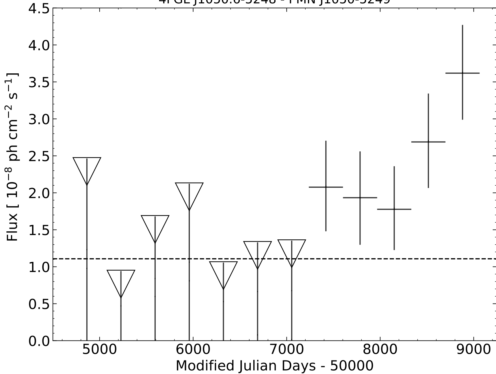
4FGL J1050.6-5248 - PMN J1050-5249
