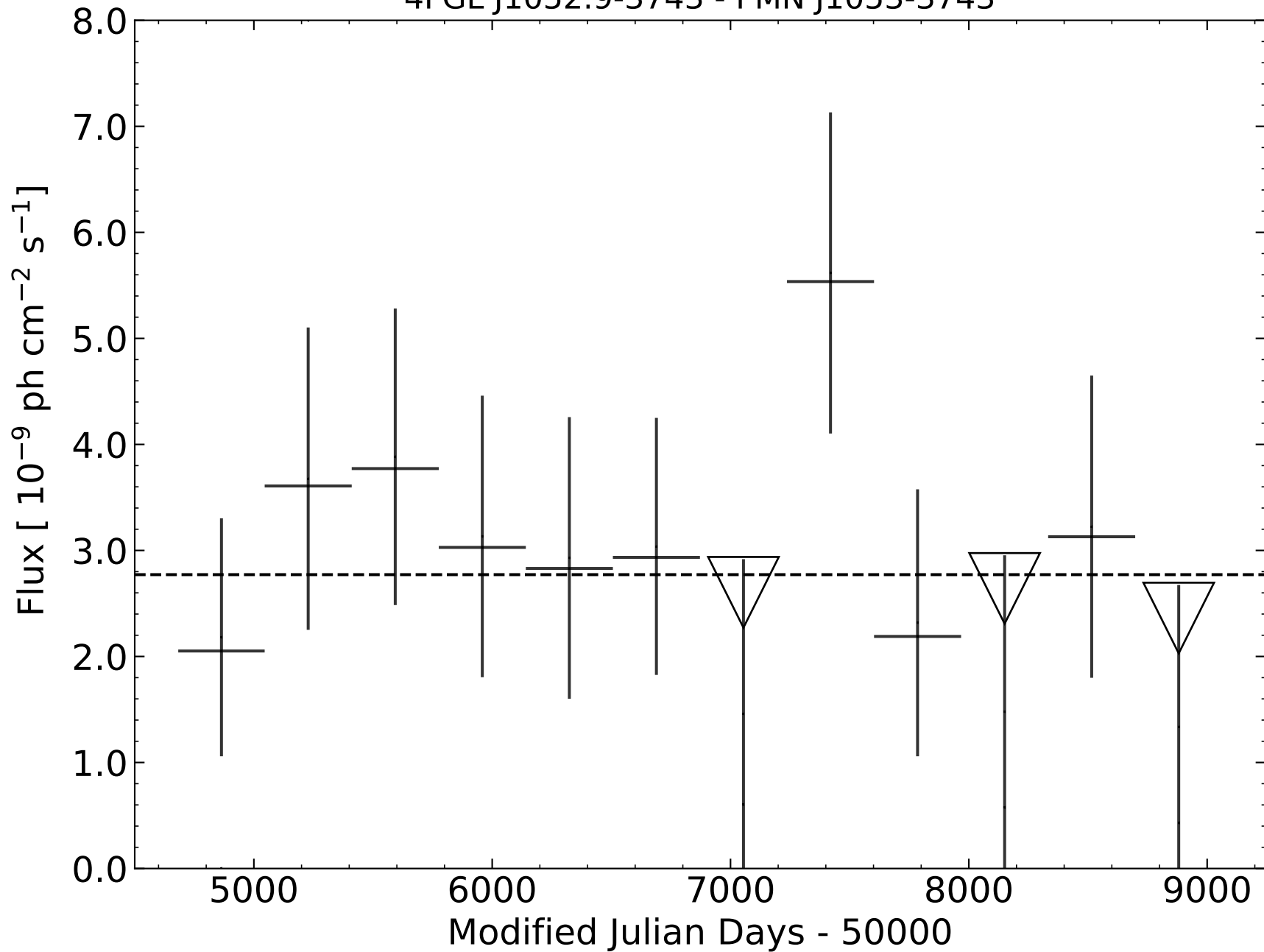
4FGL J1052.9-3743 - PMN J1053-3743
