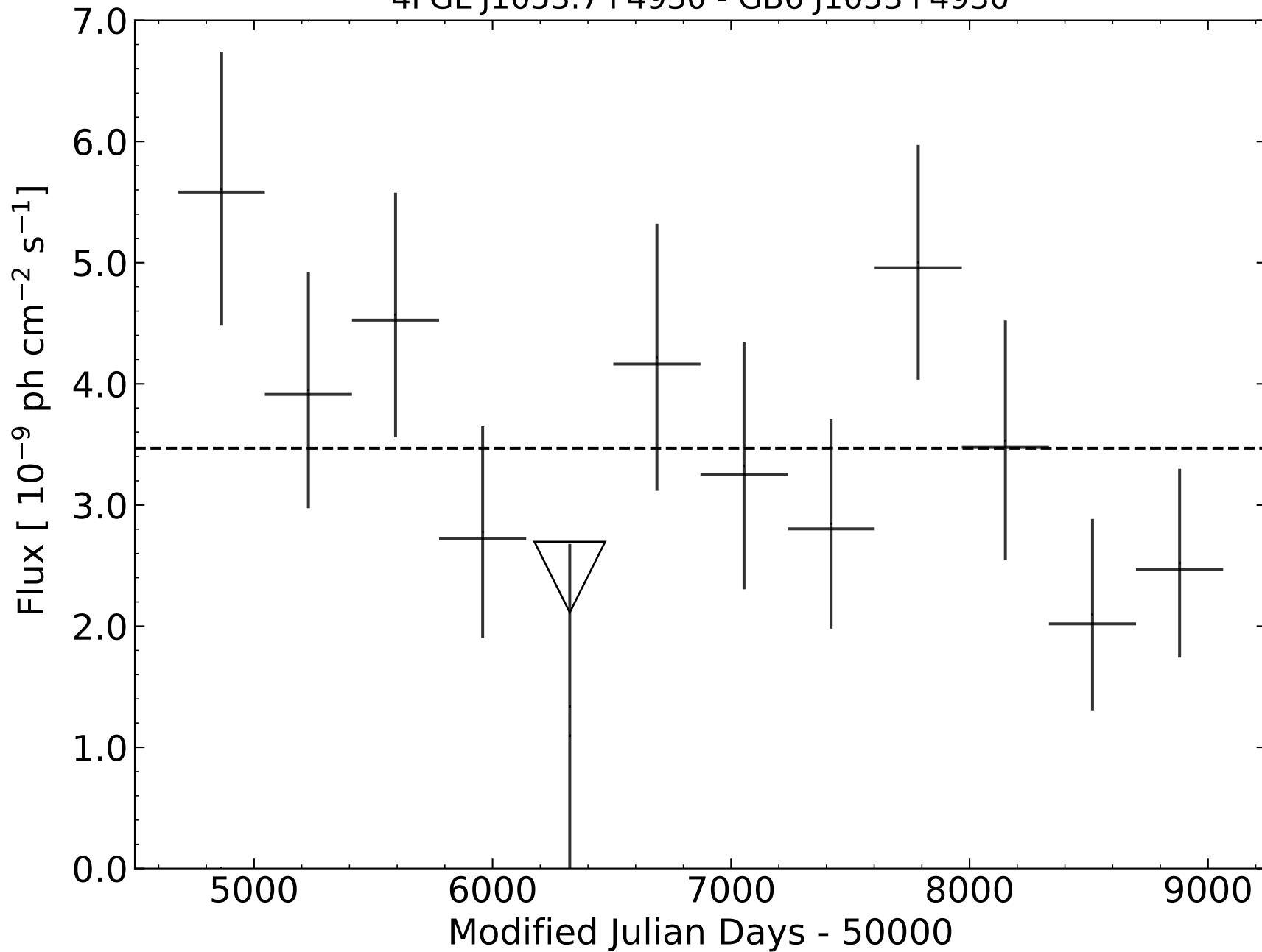
4FGL J1053.7+4930 - GB6 J1053+4930
