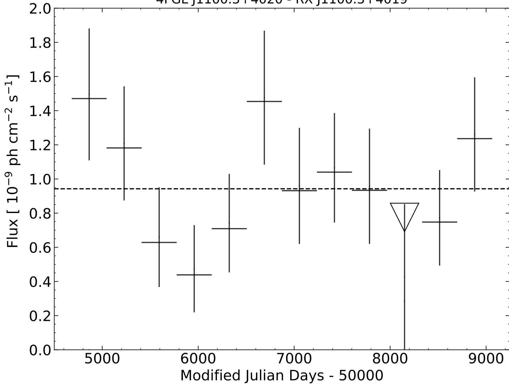
4FGL J1100.3+4020 - RX J1100.3+4019
