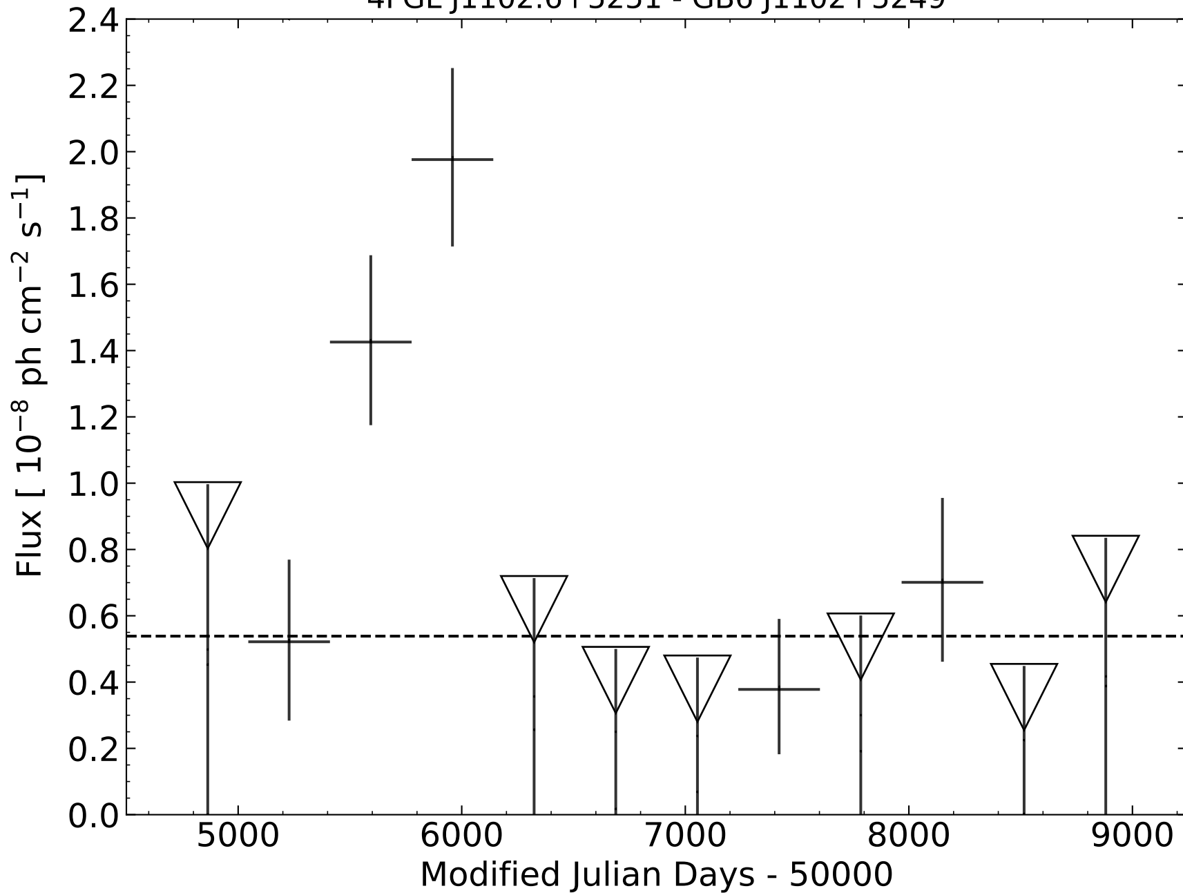
4FGL J1102.6+5251 - GB6 J1102+5249
