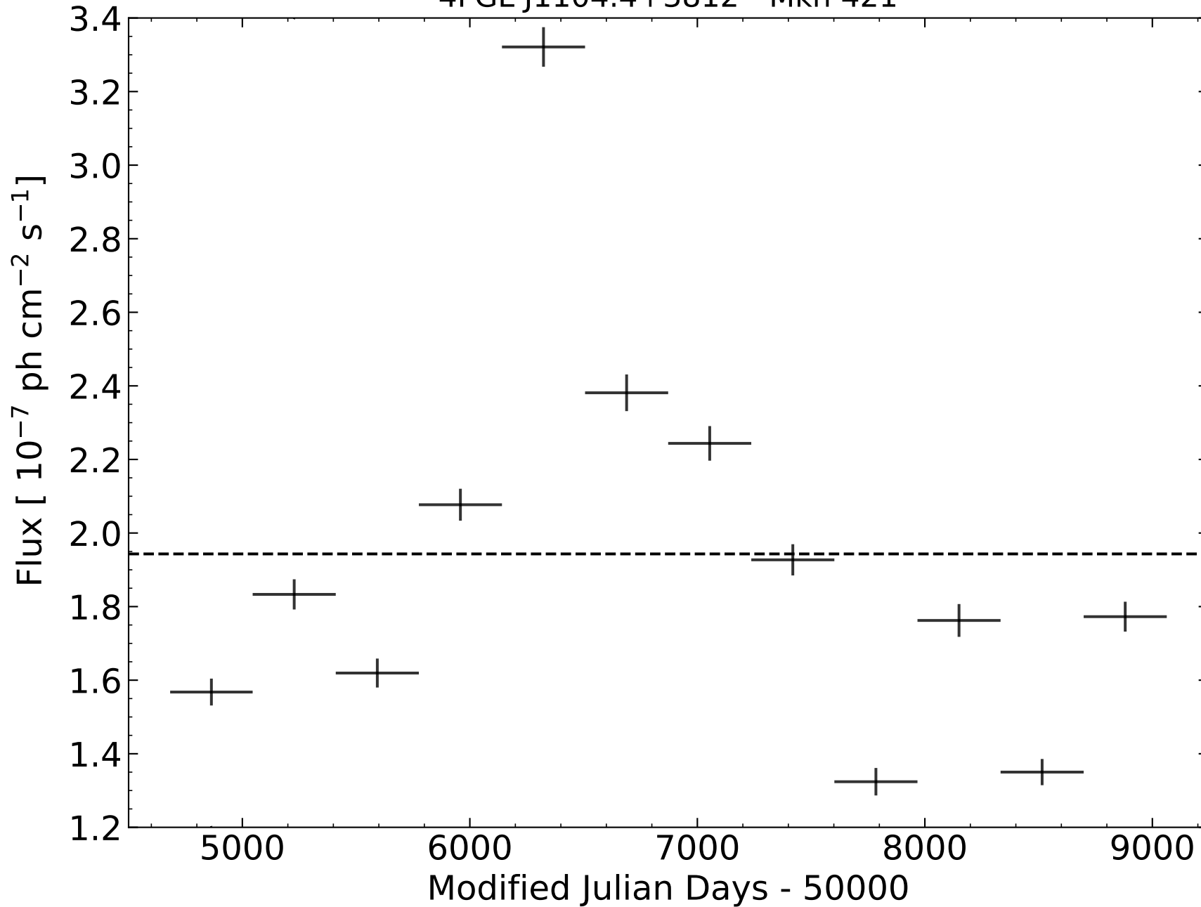
4FGL J1104.4+3812 - Mkn 421
