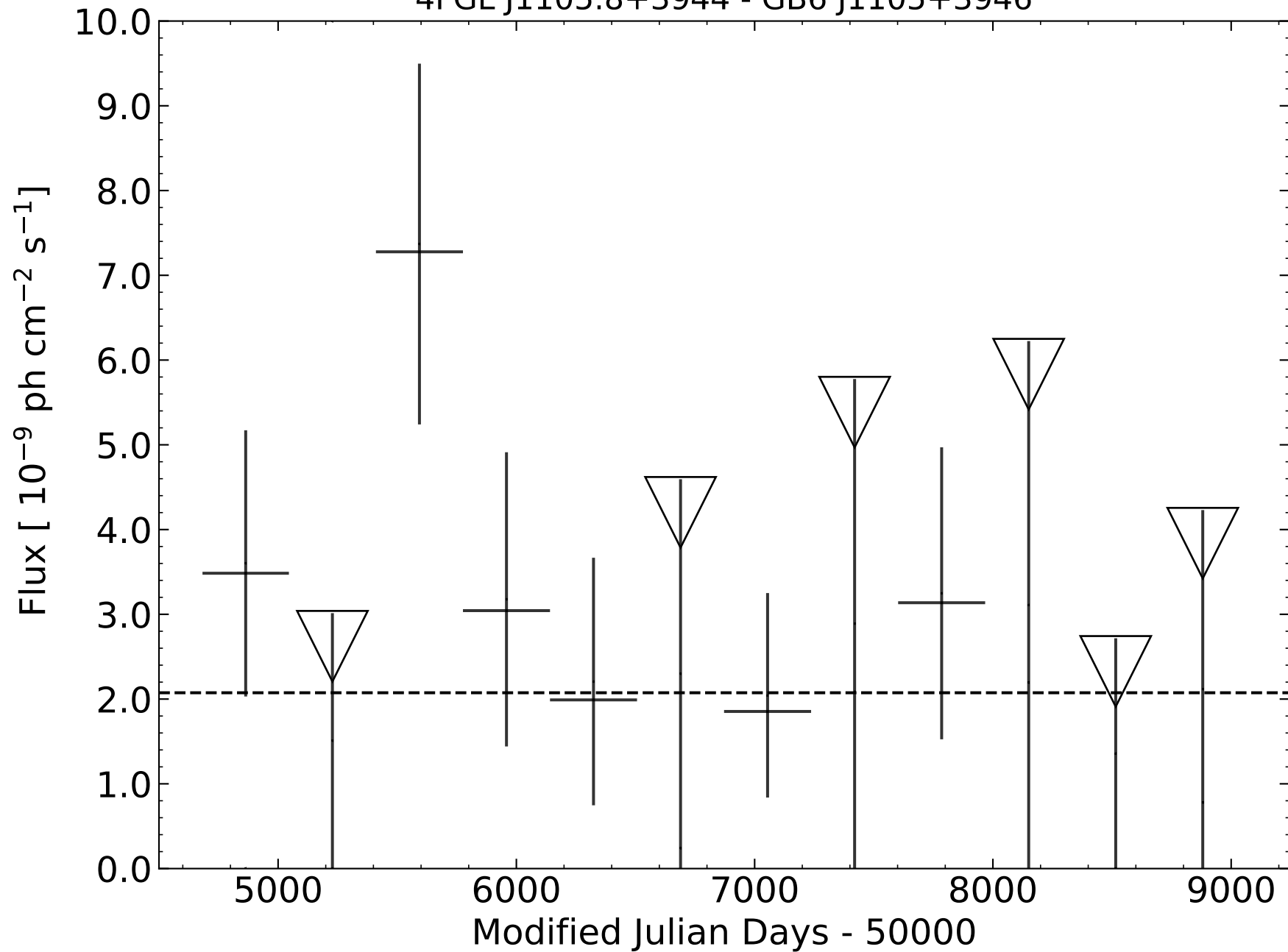
4FGL J1105.8+3944 - GB6 J1105+3946
