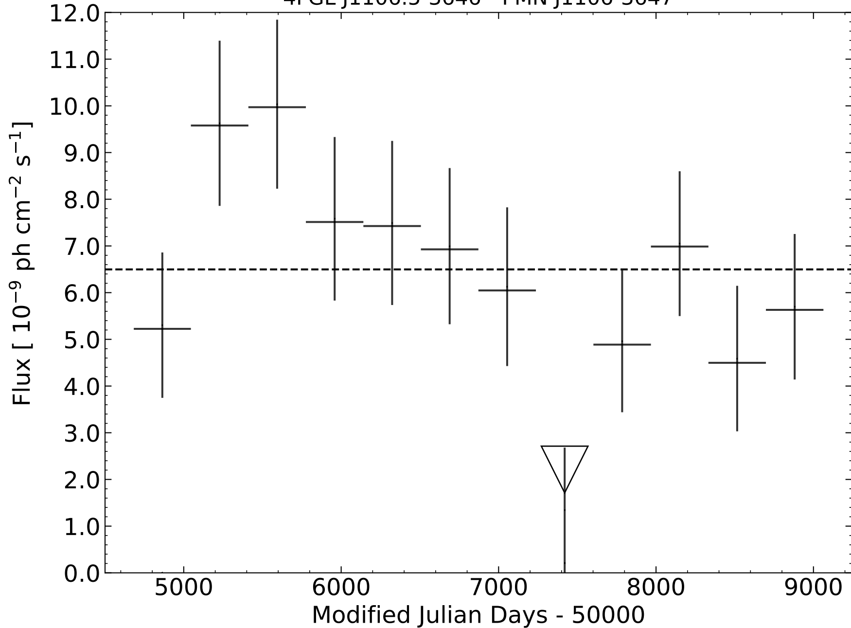
4FGL J1106.5-3646 - PMN J1106-3647
