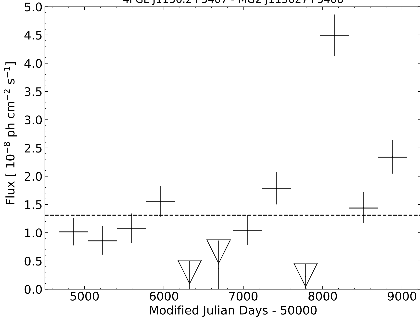
4FGL J1136.2+3407 - MG2 J113627+3408
