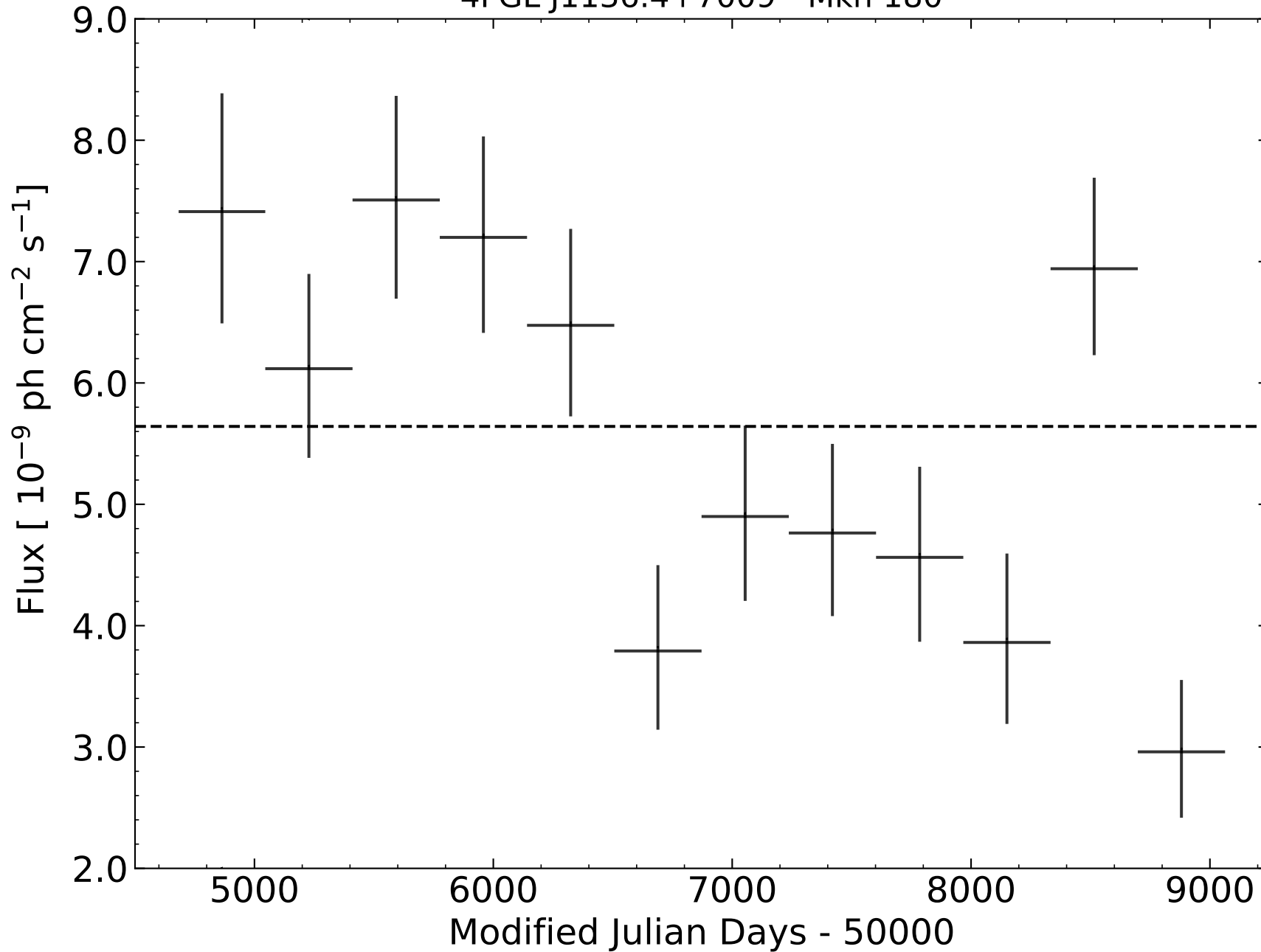
4FGL J1136.4+7009 - Mkn 180
