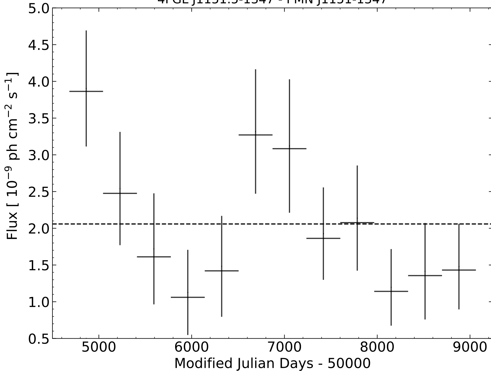
4FGL J1151.5-1347 - PMN J1151-1347
