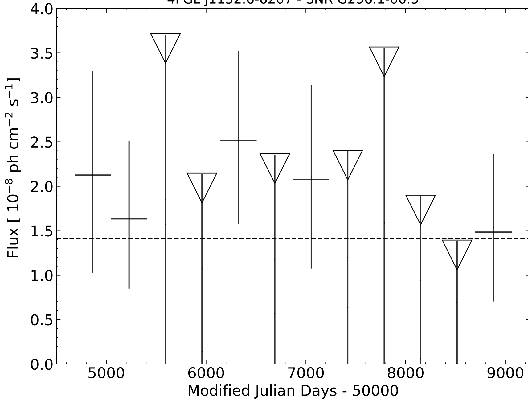
4FGL J1152.6-6207 - SNR G296.1-00.5
