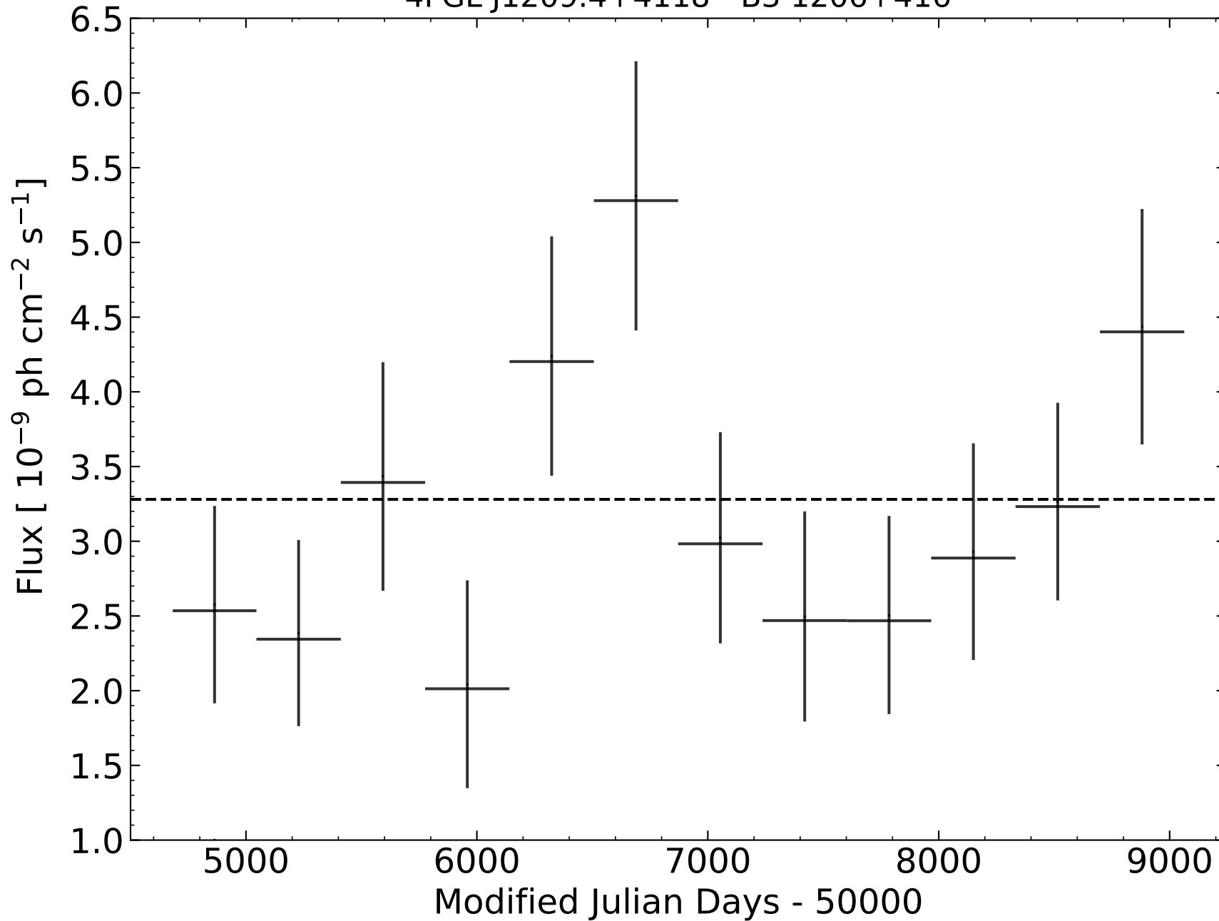
4FGL J1209.4+4118 - B3 1206+416
