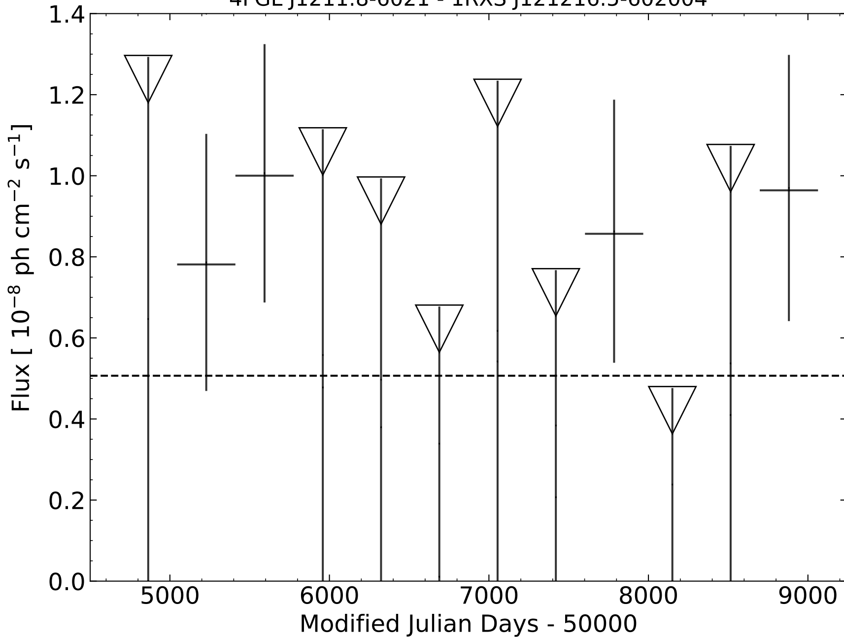
4FGL J1211.8-6021 - 1RXS J121216.5-602004
