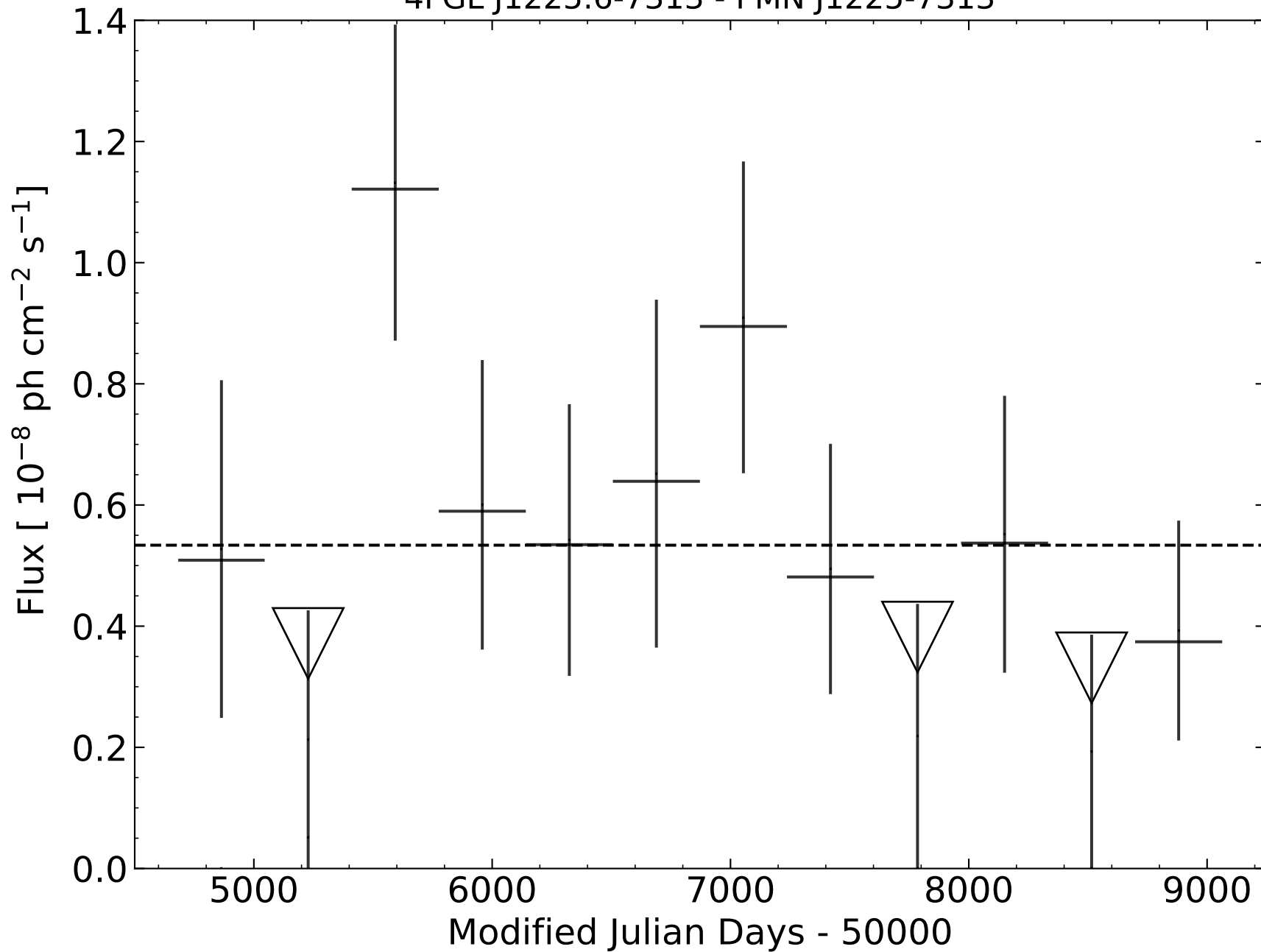
4FGL J1225.6-7313 - PMN J1225-7313
