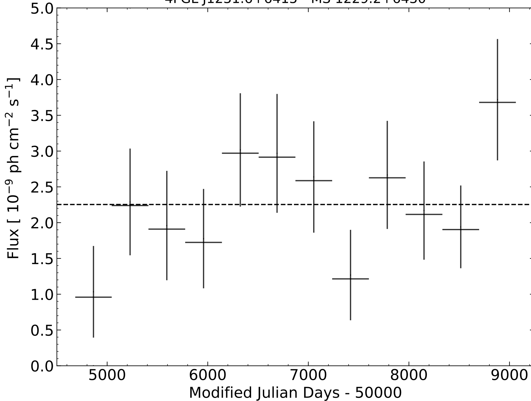
4FGL J1231.6+6415 - MS 1229.2+6430
