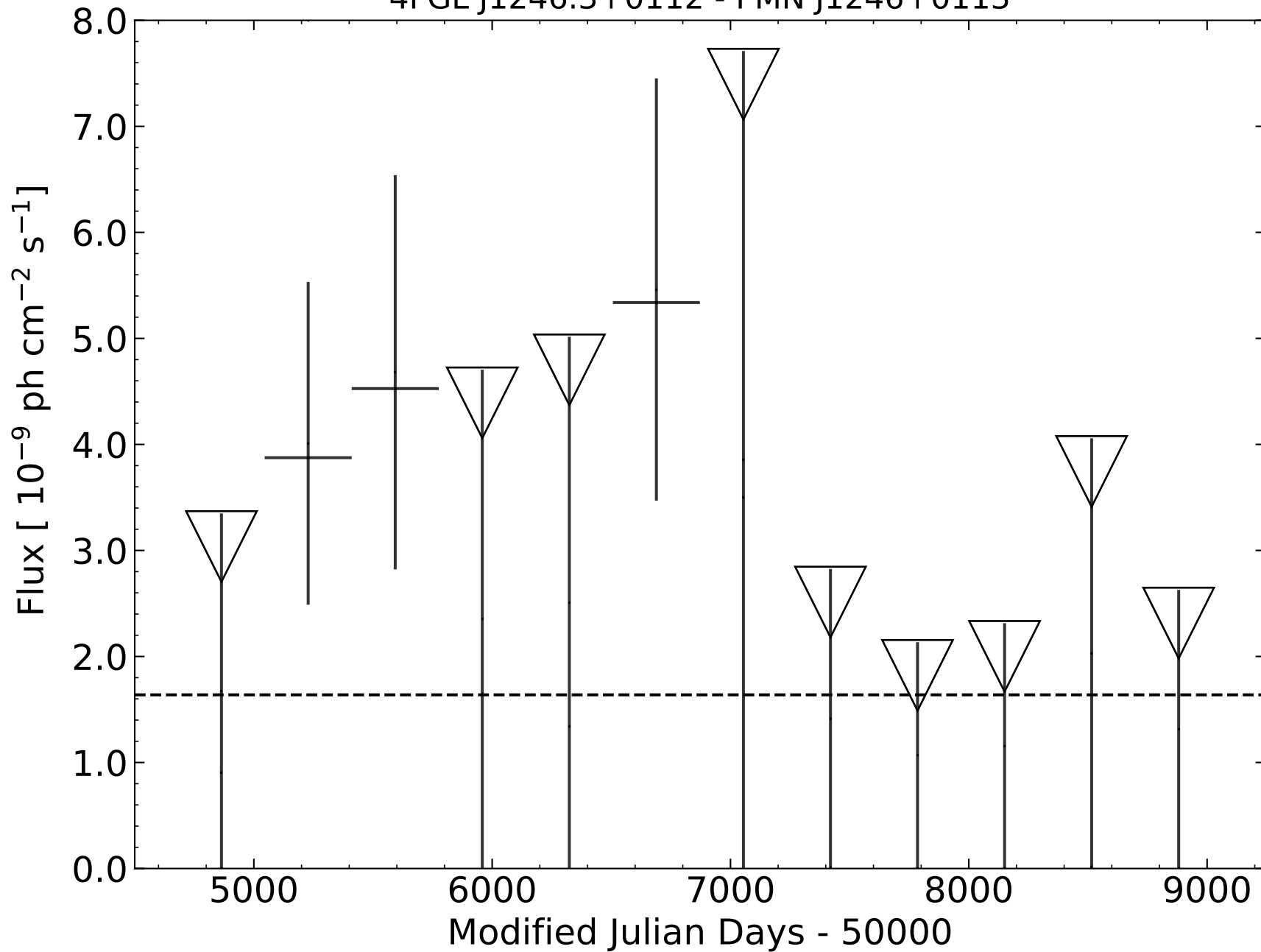
4FGL J1246.3+0112 - PMN J1246+0113
