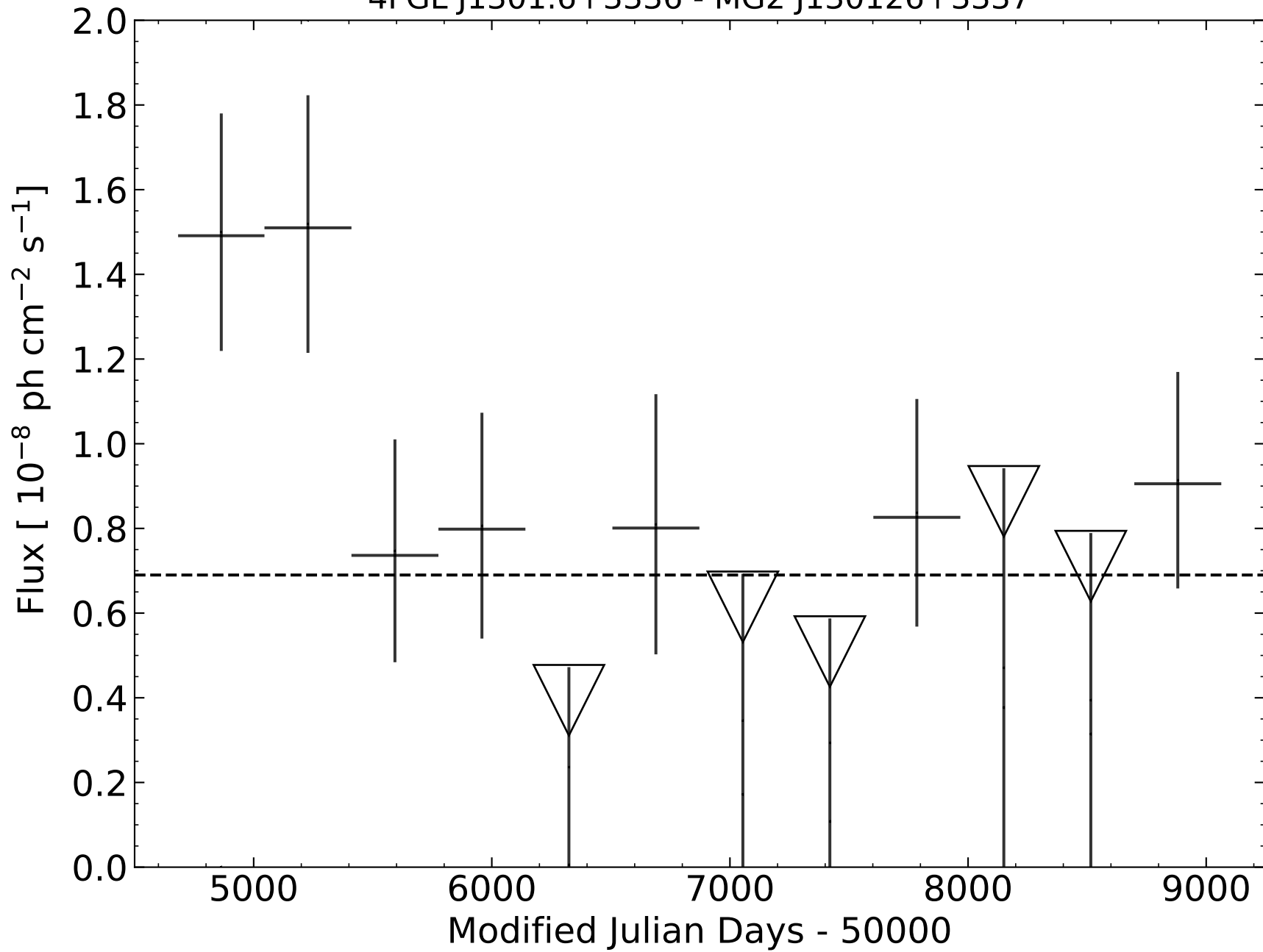
4FGL J1301.6+3336 - MG2 J130126+3337
