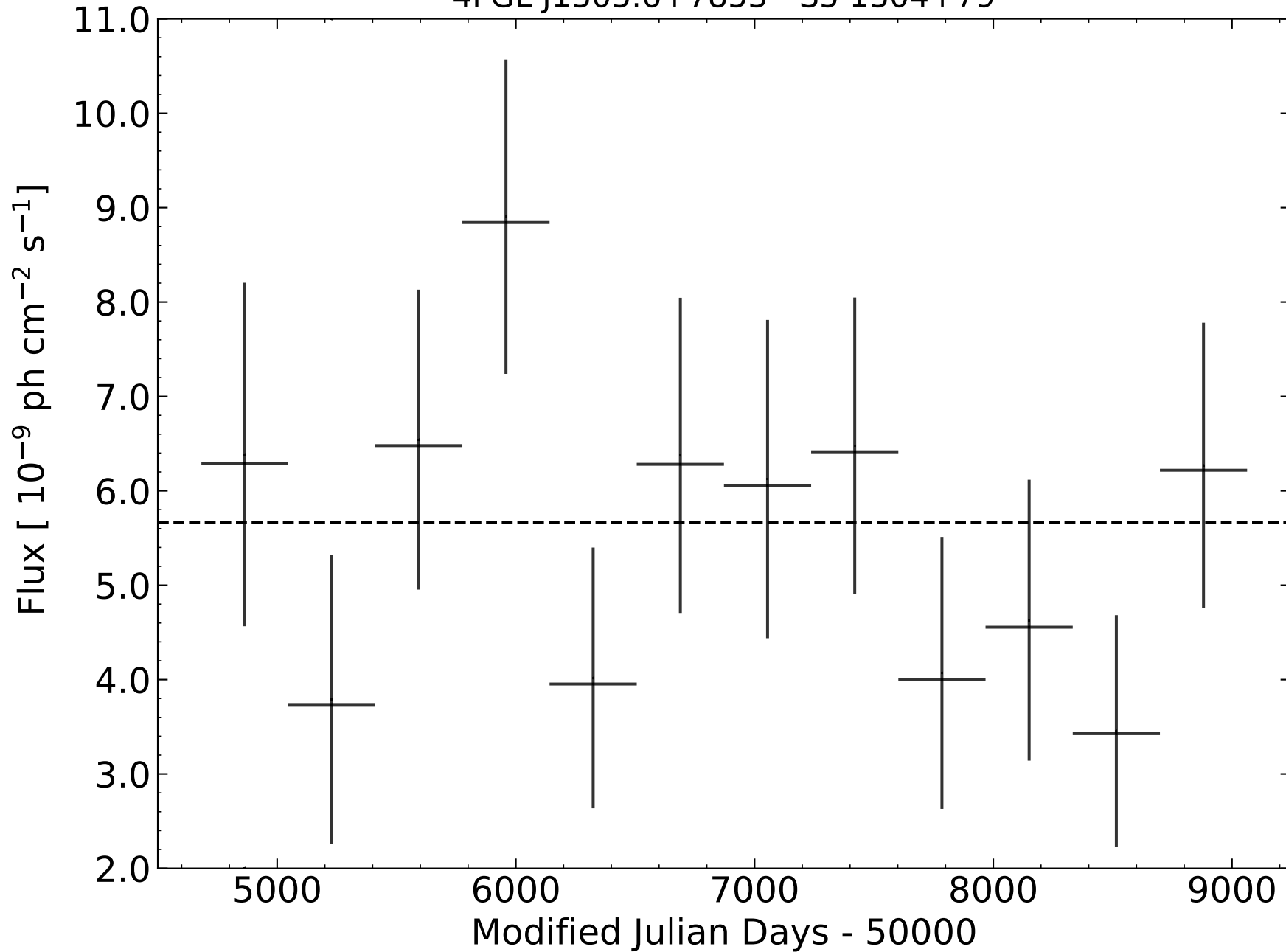
4FGL J1305.6+7853 - S5 1304+79
