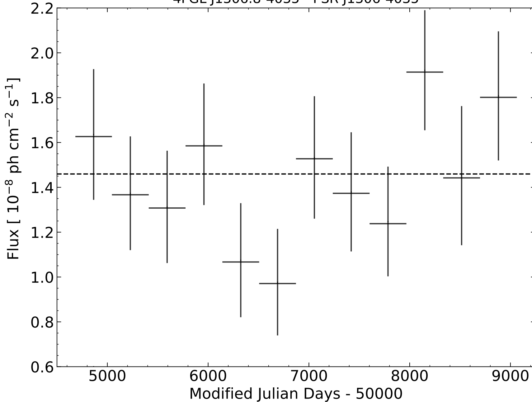
4FGL J1306.8-4035 - PSR J1306-4035
