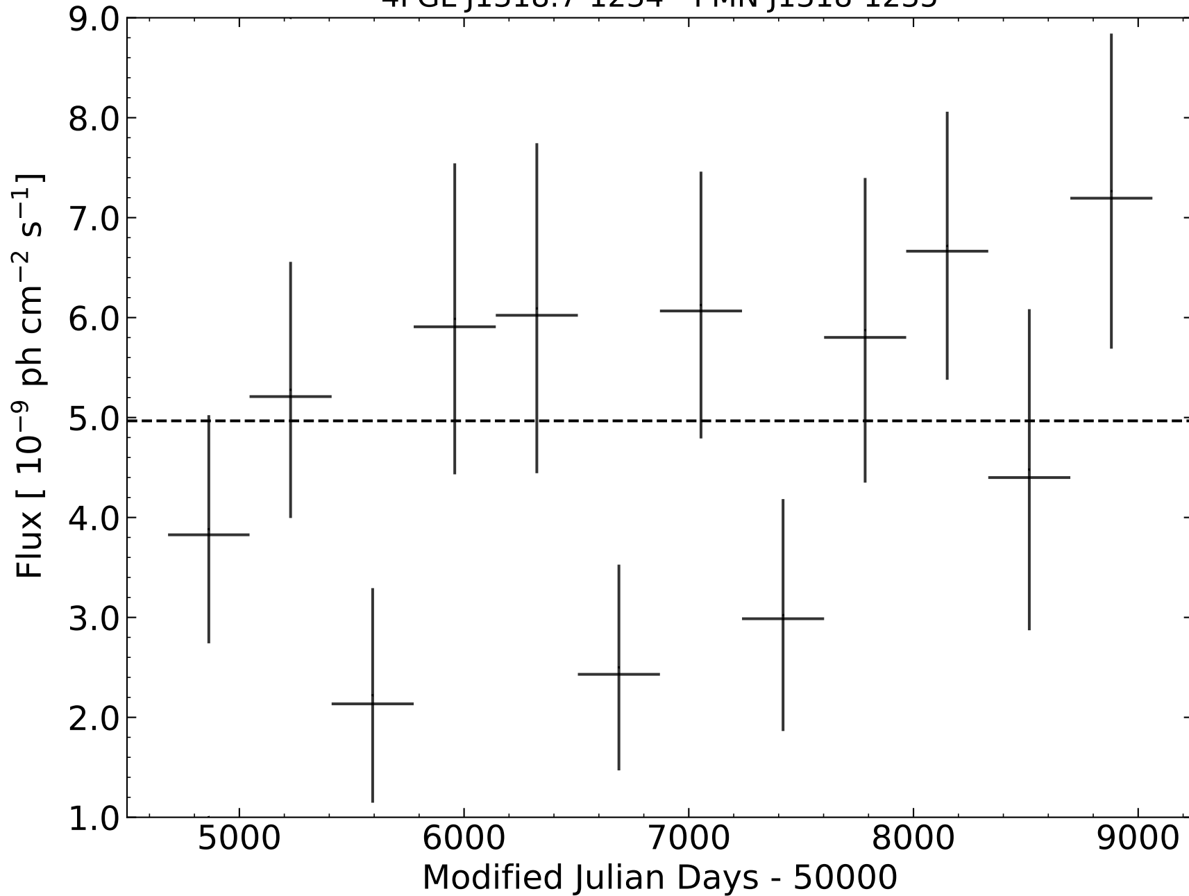
4FGL J1318.7-1234 - PMN J1318-1235
