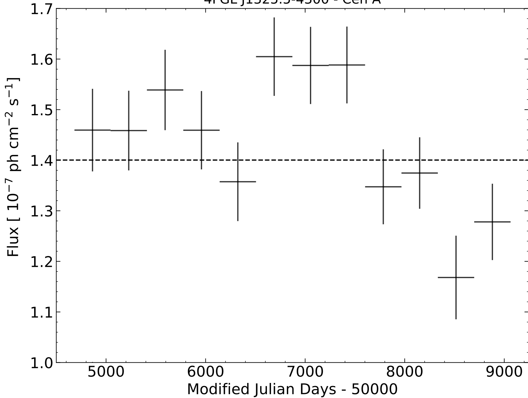
4FGL J1325.5-4300 - Cen A
