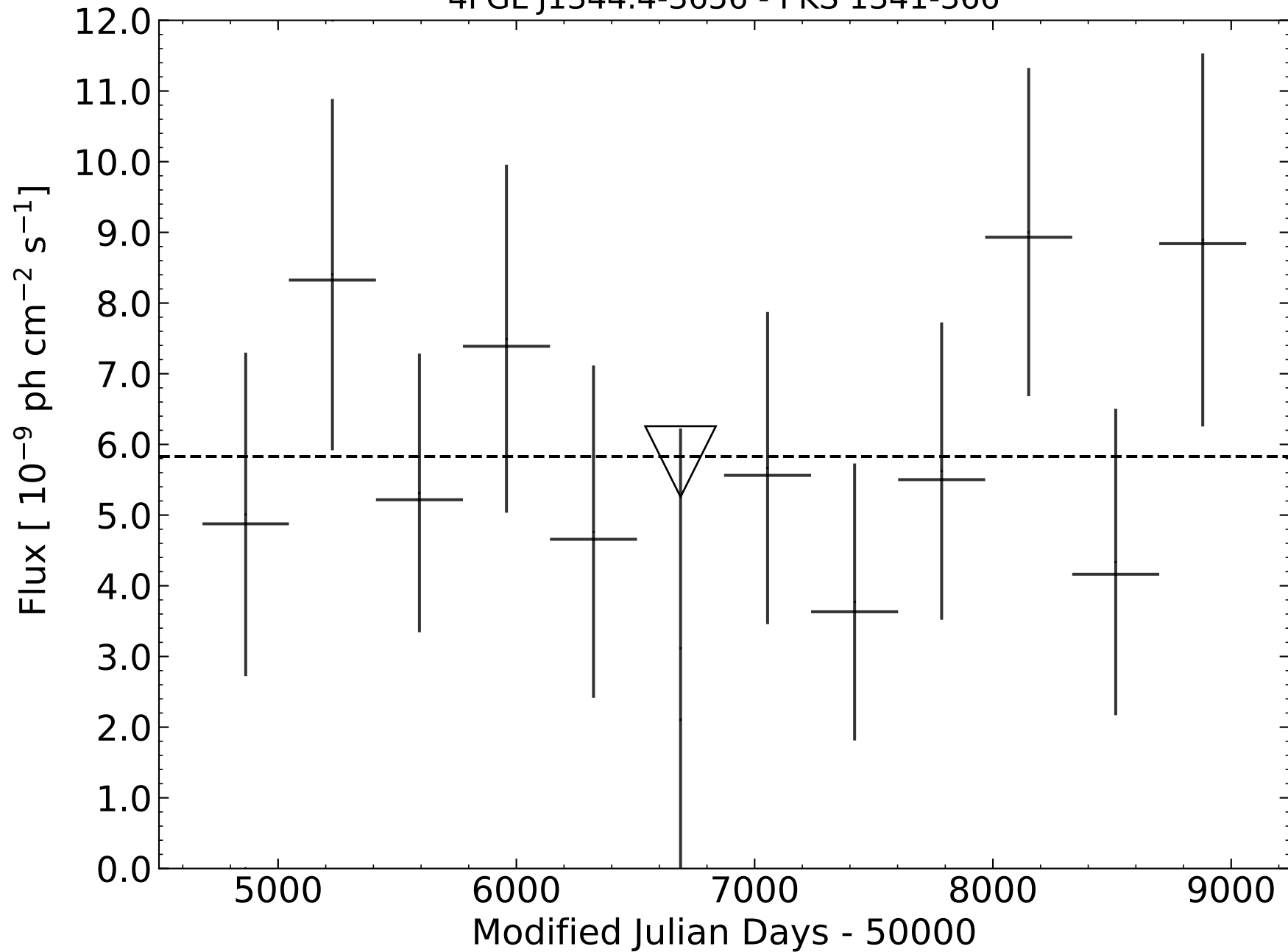
4FGL J1344.4-3656 - PKS 1341-366
