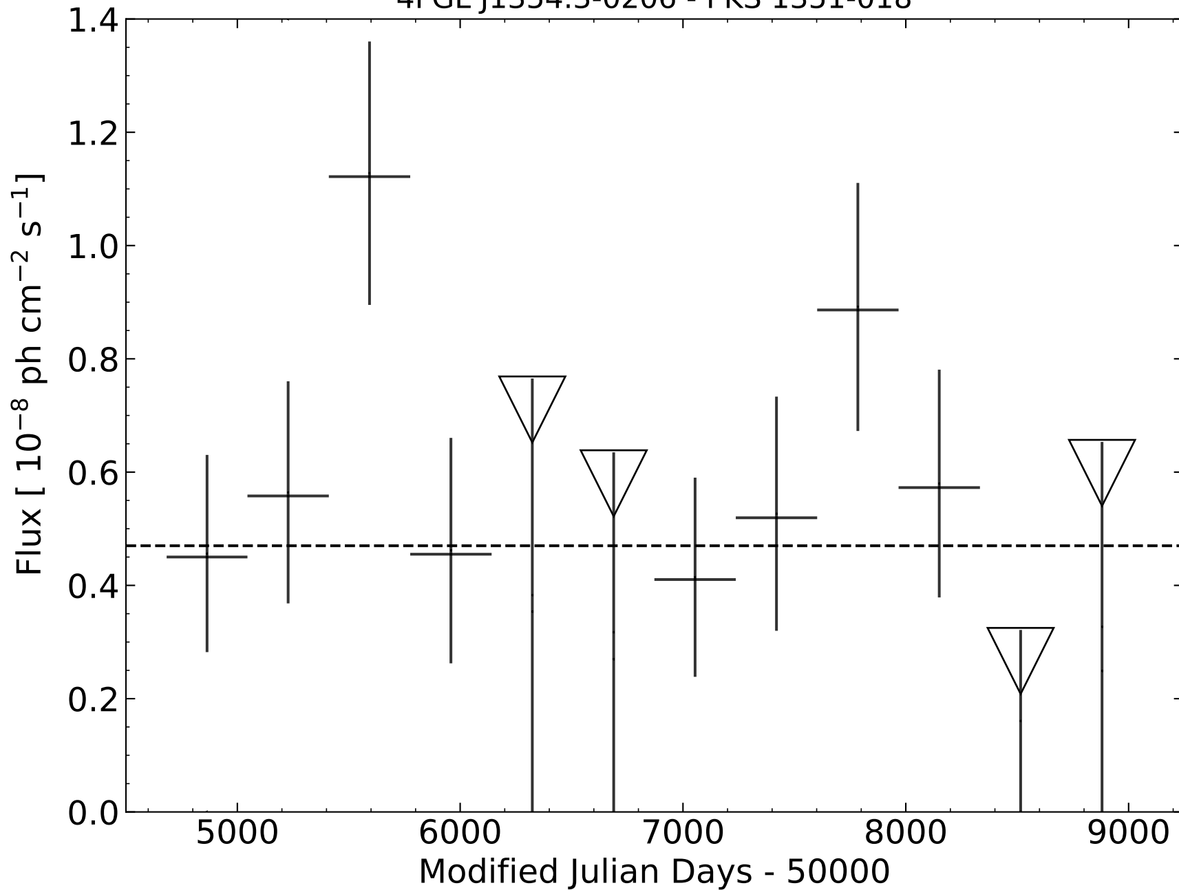
4FGL J1354.3-0206 - PKS 1351-018
