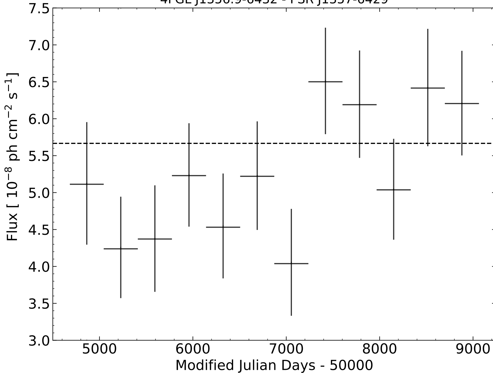
4FGL J1356.9-6432 - PSR J1357-6429
