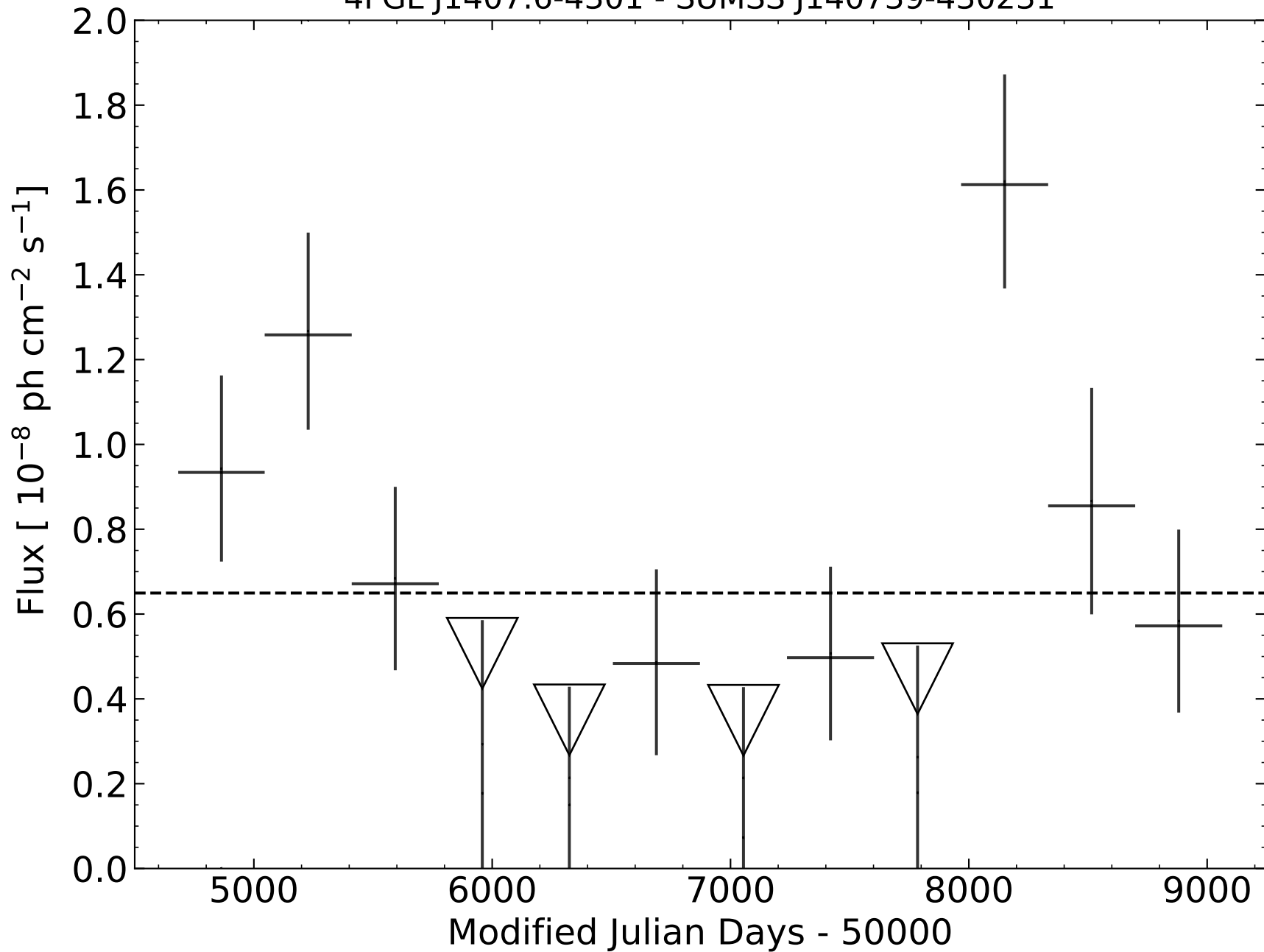
4FGL J1407.6-4301 - SUMSS J140739-430231
