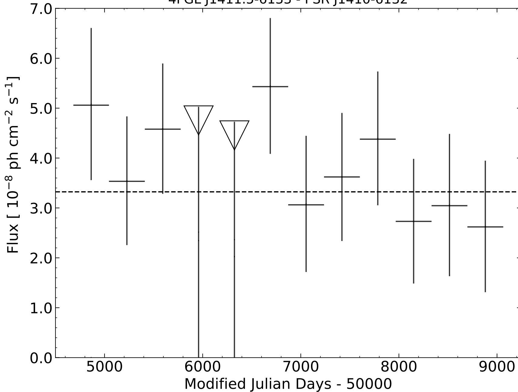
4FGL J1411.5-6133 - PSR J1410-6132
