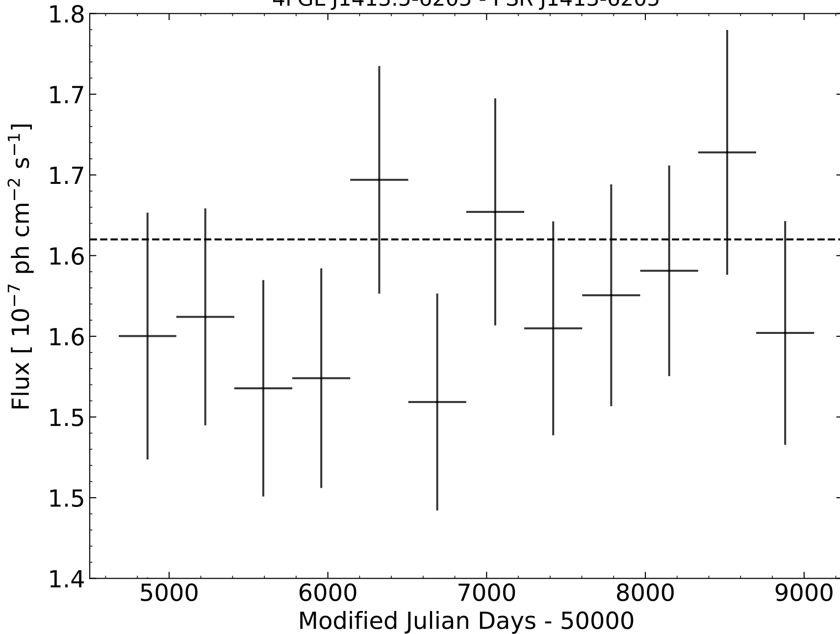
4FGL J1413.5-6205 - PSR J1413-6205
