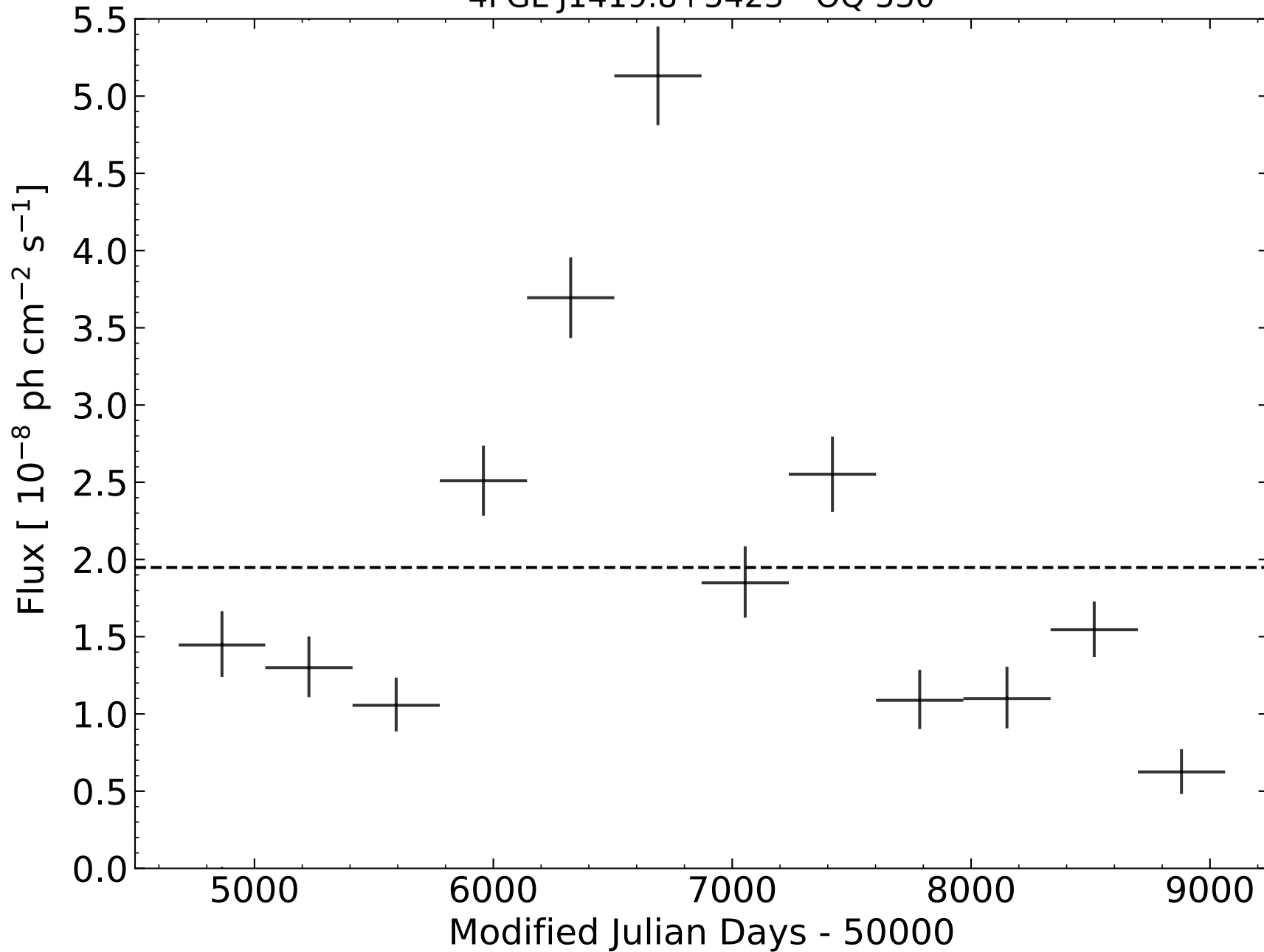
4FGL J1419.8+5423 - OQ 530
