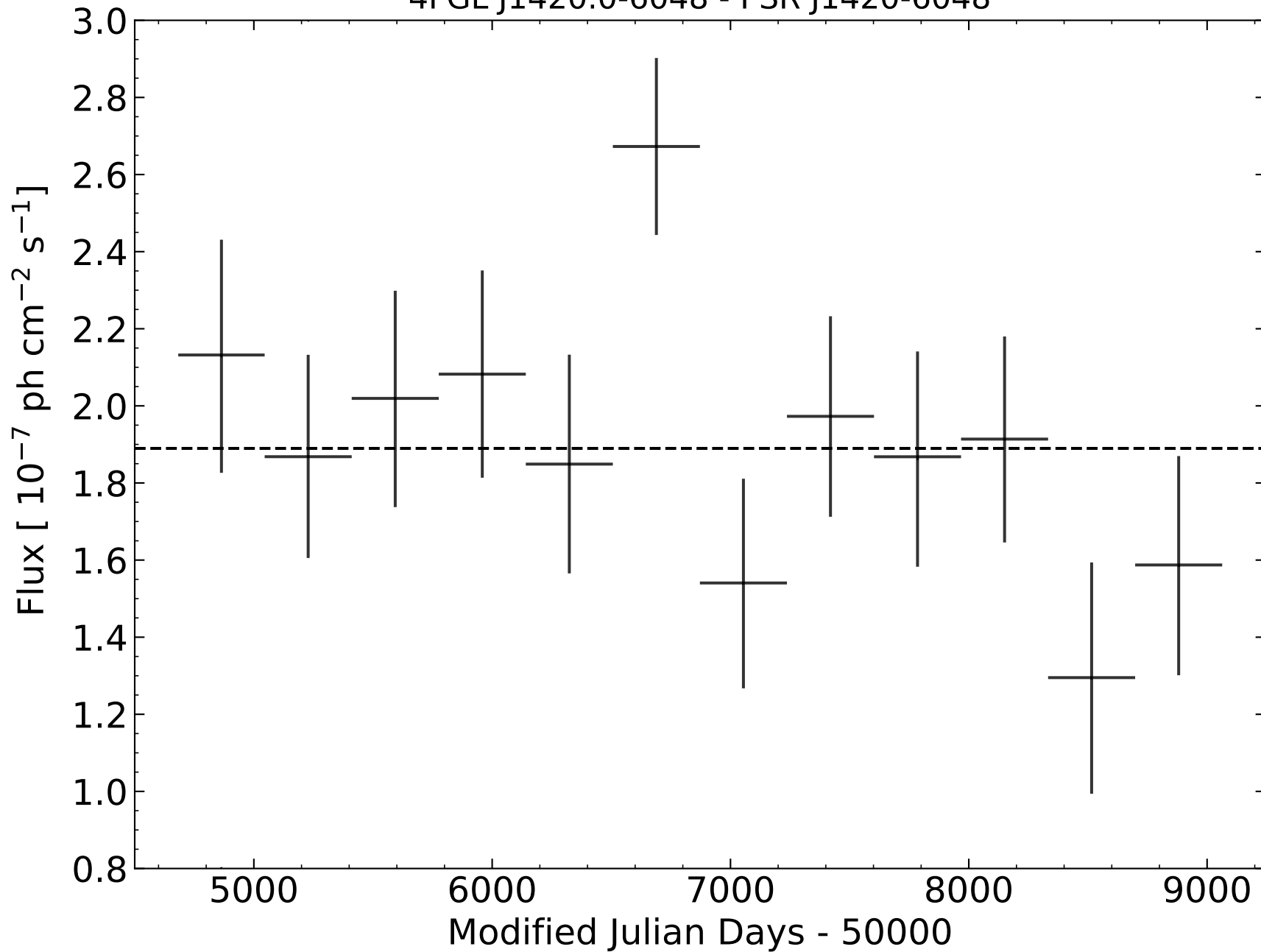
4FGL J1420.0-6048 - PSR J1420-6048
