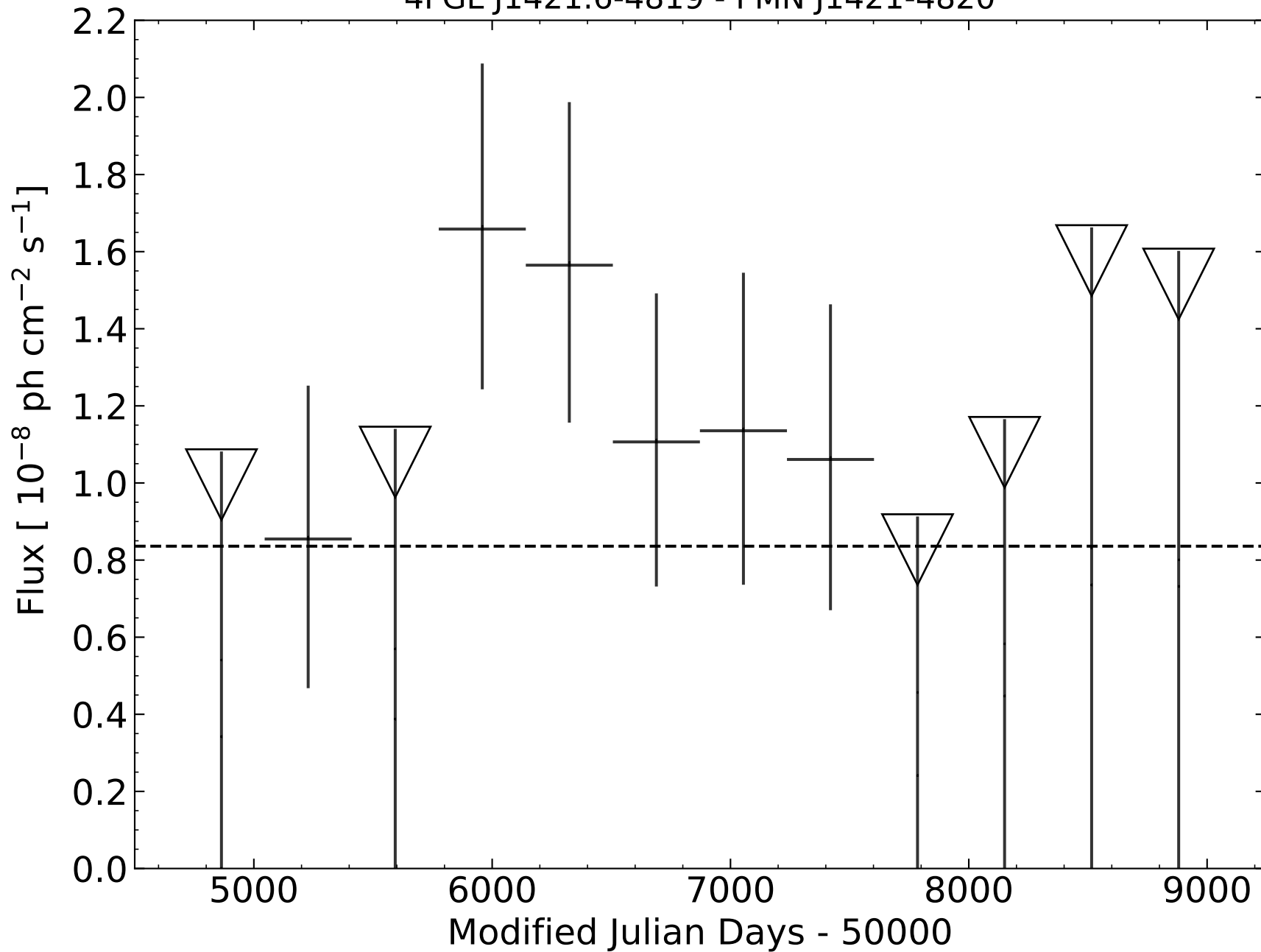
4FGL J1421.6-4819 - PMN J1421-4820
