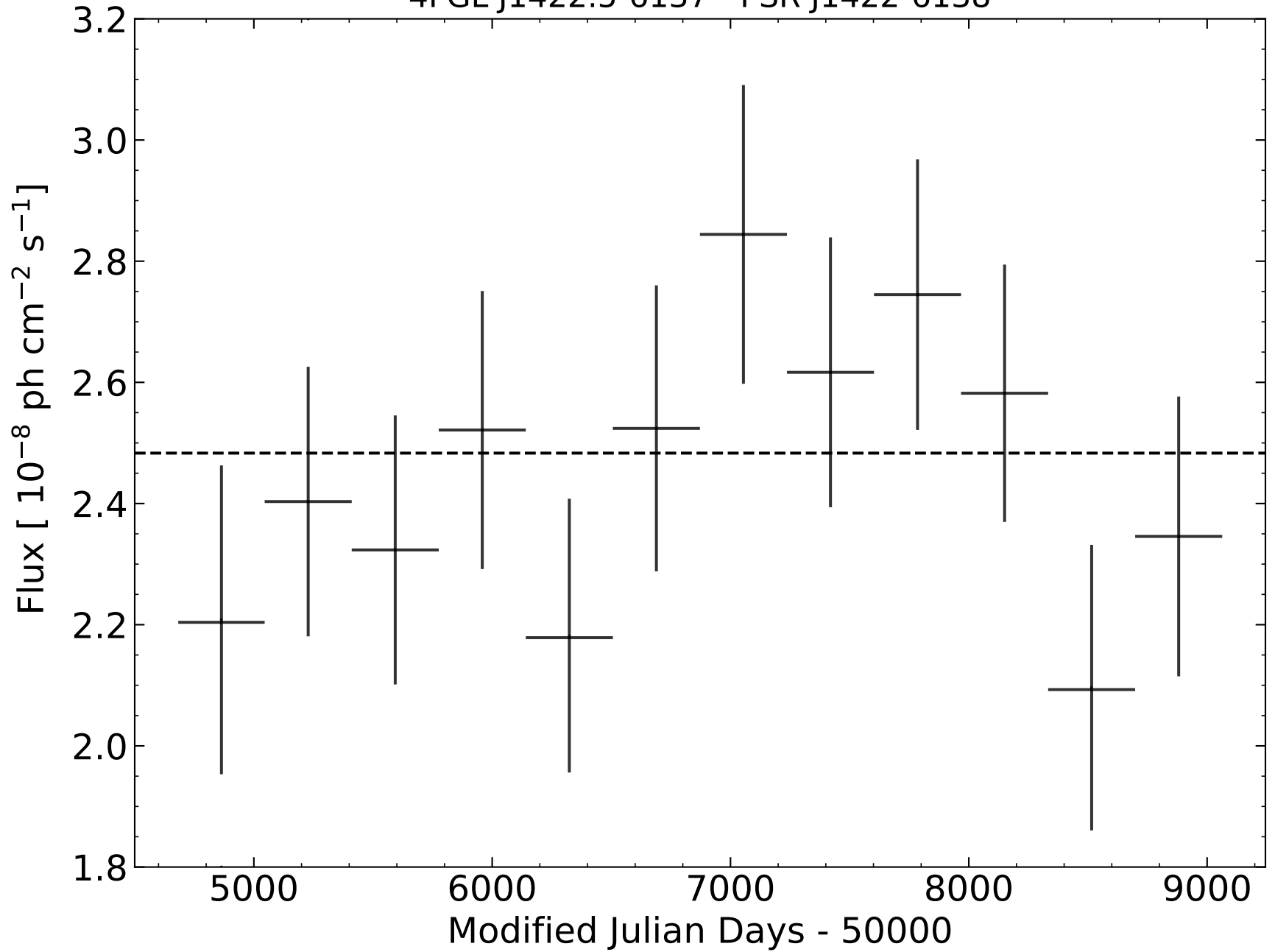
4FGL J1422.5-6137 - PSR J1422-6138
