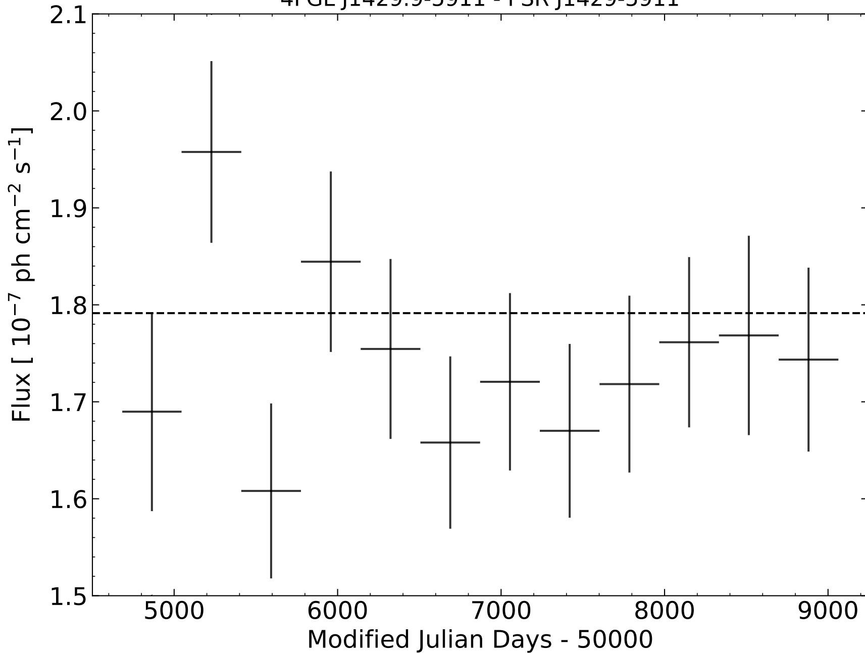
4FGL J1429.9-5911 - PSR J1429-5911
