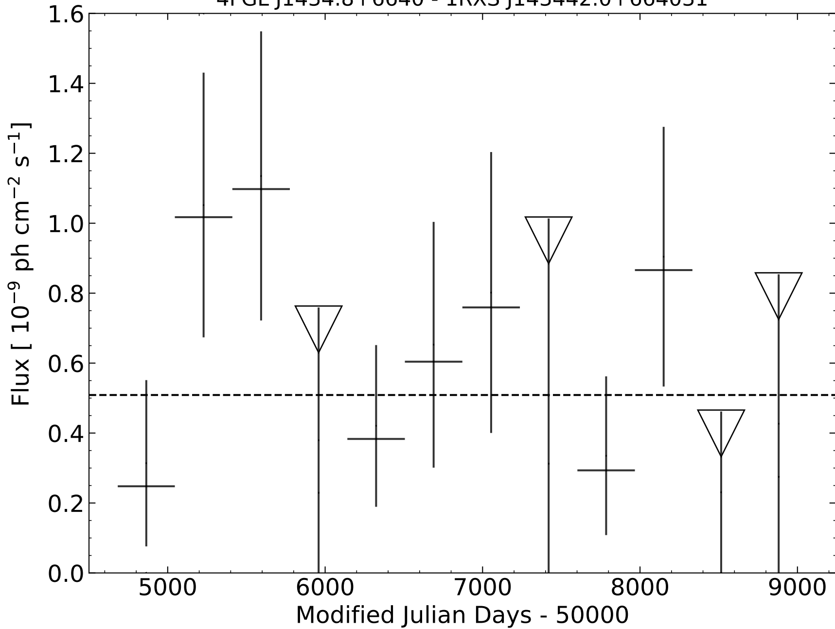
4FGL J1434.8+6640 - 1RXS J143442.0+664031
