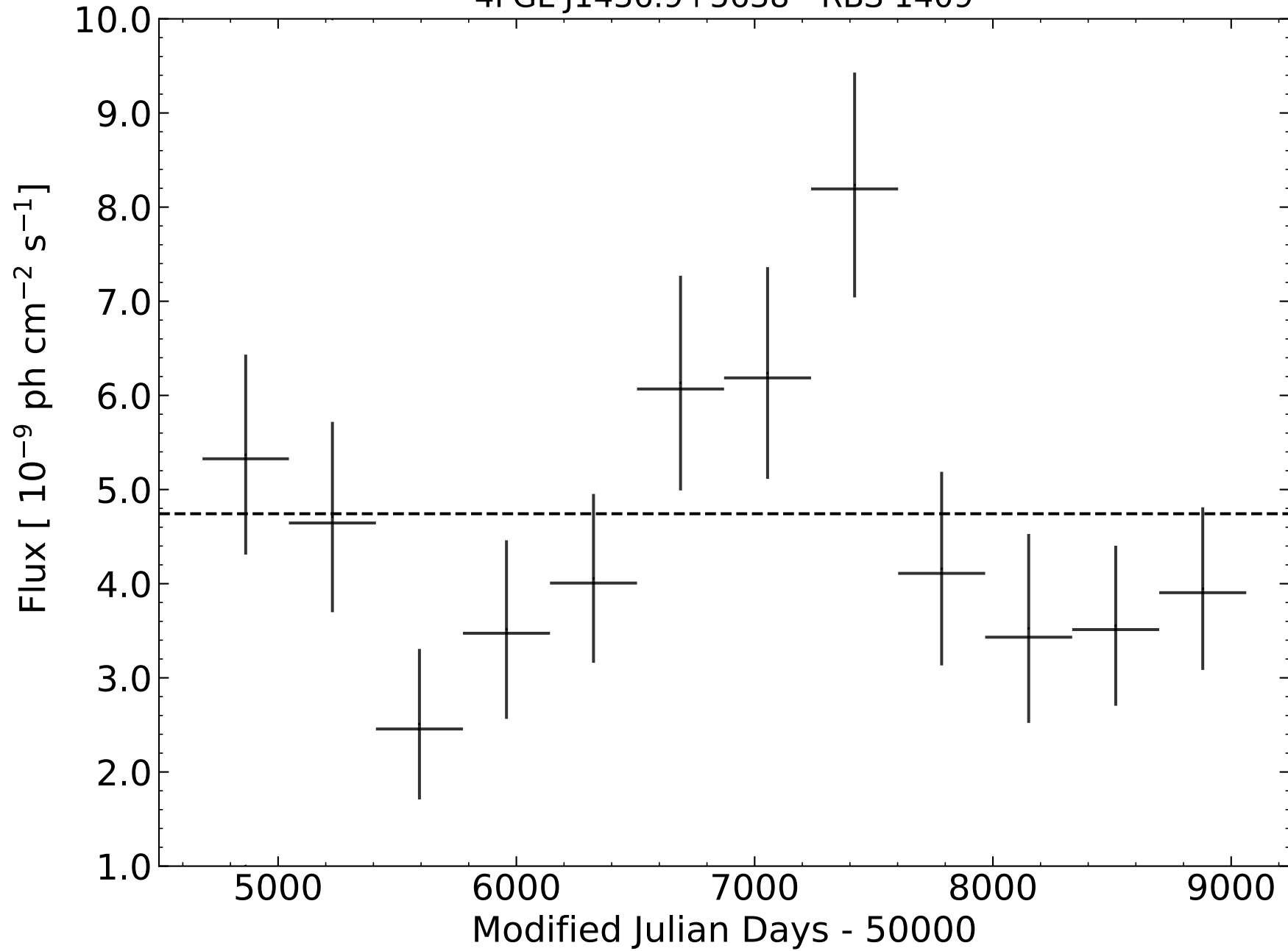
4FGL J1436.9+5638 - RBS 1409
