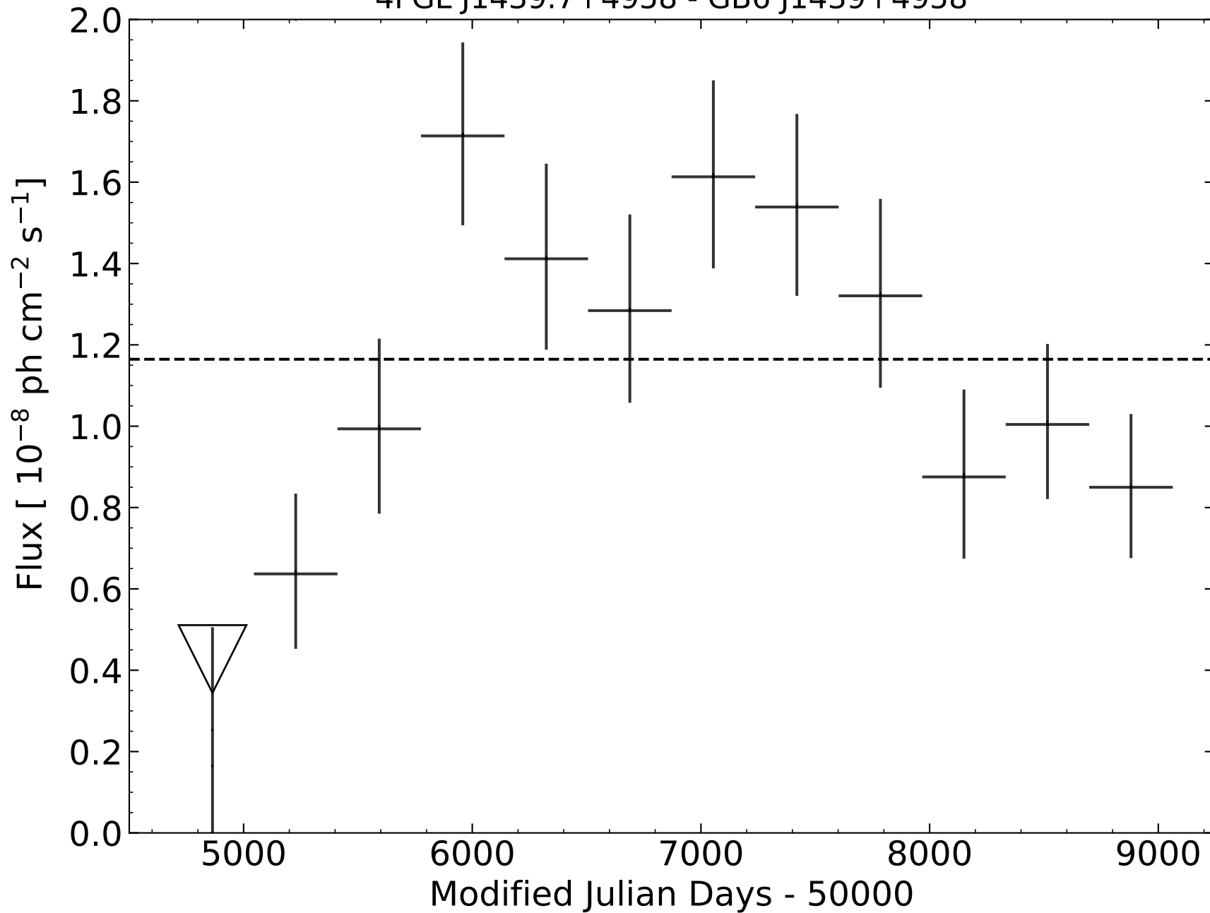
4FGL J1439.7+4958 - GB6 J1439+4958
