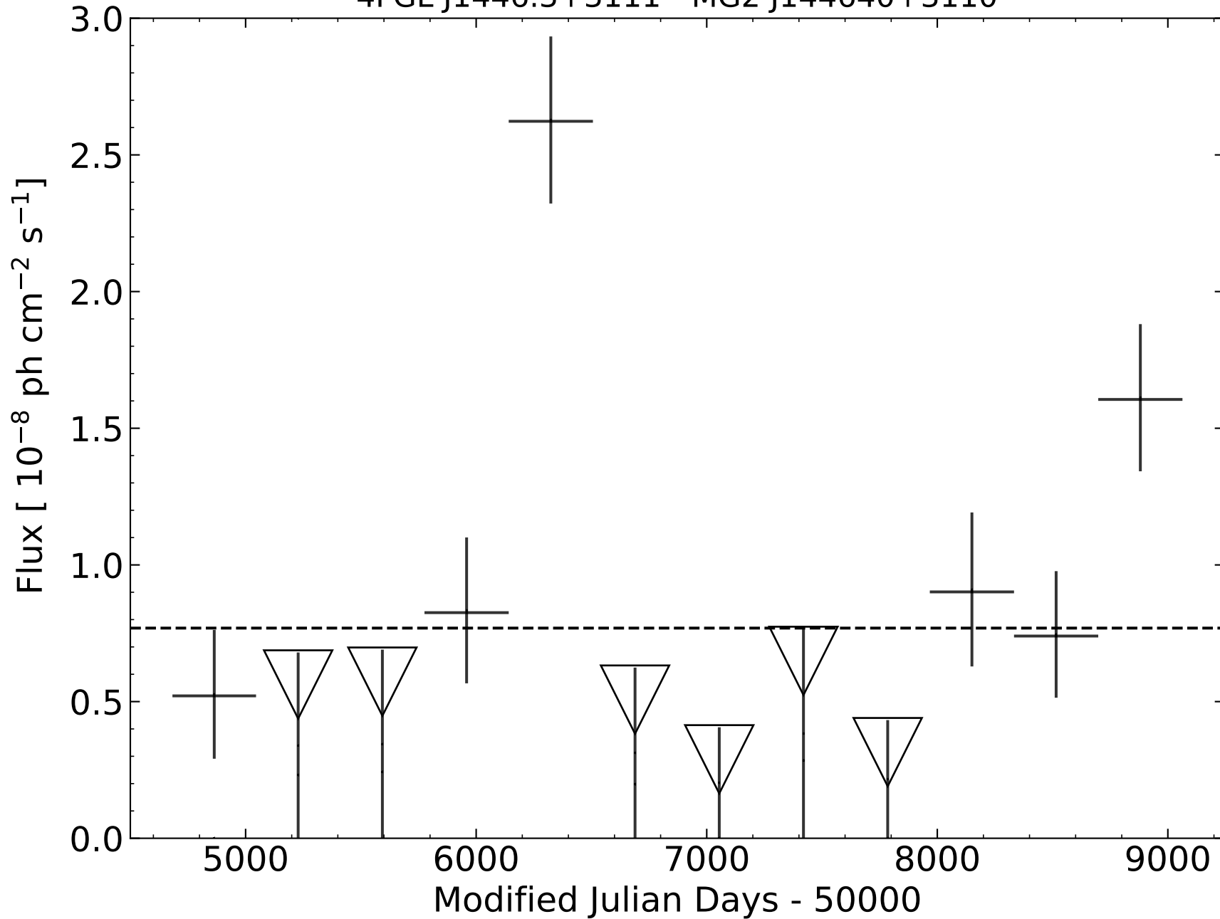
4FGL J1446.3+3111 - MG2 J144640+3110
