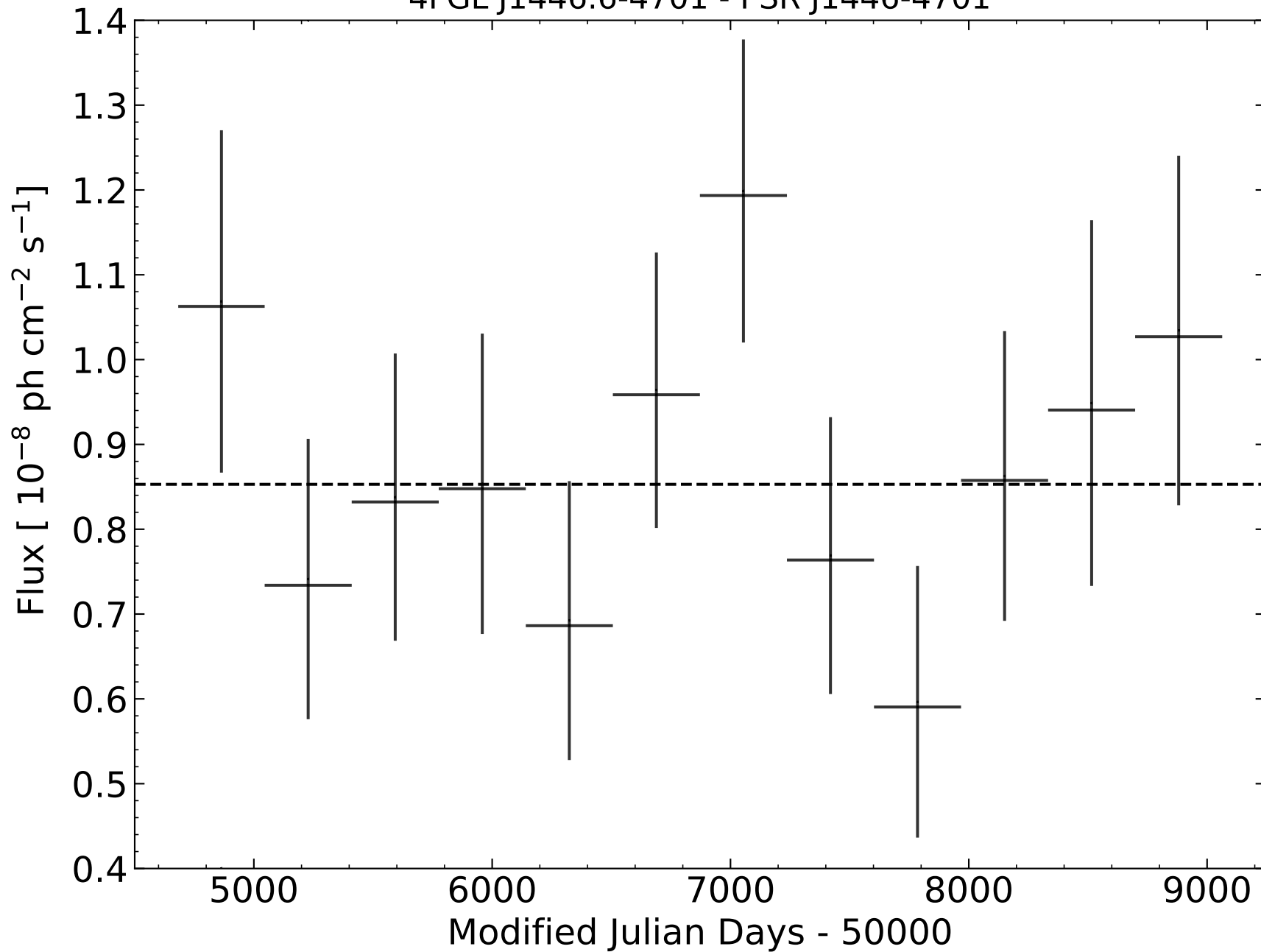
4FGL J1446.6-4701 - PSR J1446-4701
